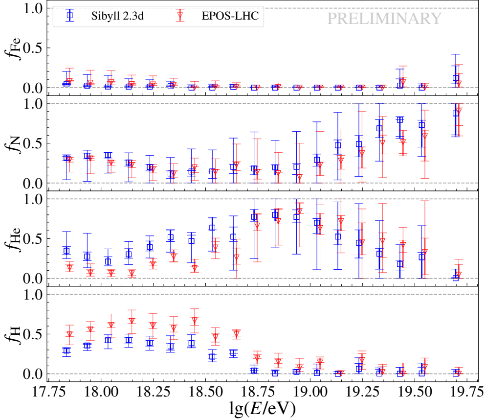
Figure 1: The mass composition fit for four elemental mass groups: H, He, N, and Fe (top four panels). The error bars denote statistical (thick cap) and total (thin cap) uncertainties.
