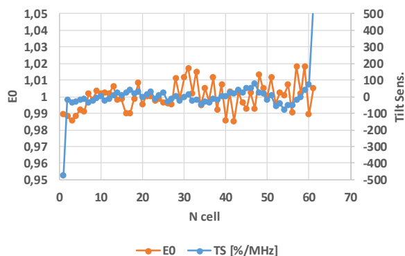
Figure 4: E0 and TS as obtained in April 2021 after the replacement of all copper tuners and PCs.
