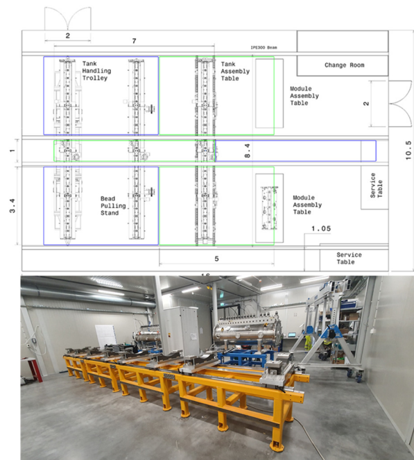
Figure 2: Sketch and picture of DTLW at ESS-Lund.
