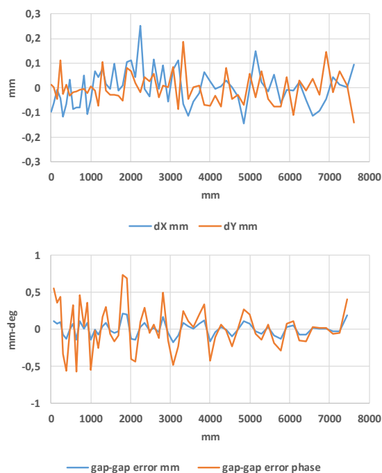
Figure 5: Gap to gap errors and PMQ transverse alignment as result of assembly of DTL1.
