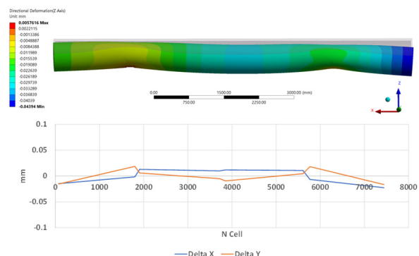
Figure 3: Simulated and measured deformation when the DTL is moved to 2 supports.
