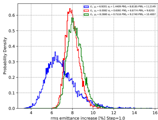
Figure 6: Emittance increase distribution at the end of the 5 DTLs with respect to nominal input beam.
