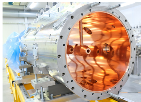
Figure 7: DTL4 - Module4 assembled at ESS Lund.
