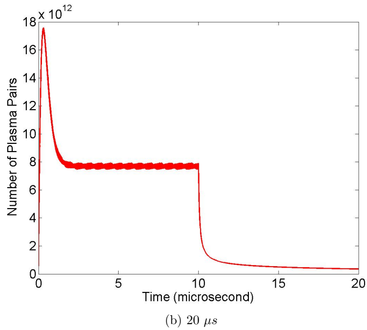
Figure 5.16: Simulated values of number of electrons in the HPRF cavity filled with pure hydrogen gas at 100 atm.
