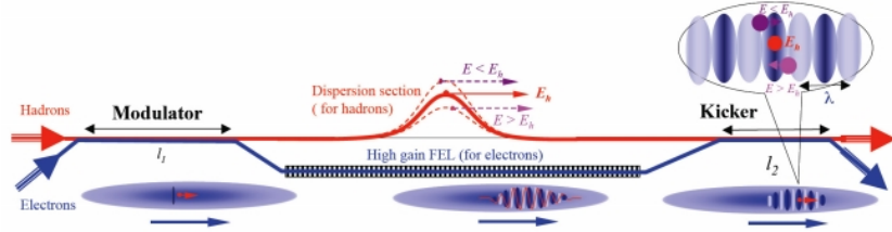
Figure 6.1: General schematic of the Coherent Electron Cooling [44].
