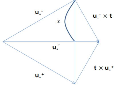
Figure 2.11: Geometric Relations
