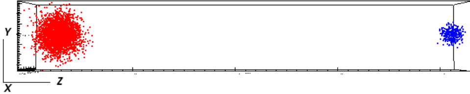
Figure 4.1: Code Validation
