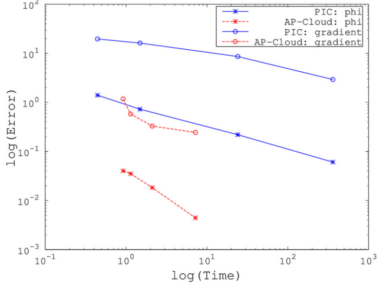
Figure 2.6: Dependence of errors on time for PIC and AP-Cloud in 2D Gaussian halo problem [7].
