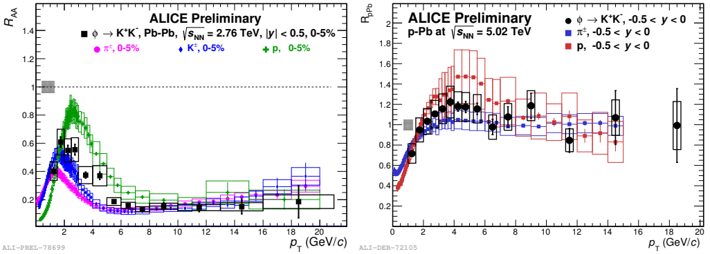
Figure 3. Nuclear modification factor of \phi in 0-5% central Pb–Pb collisions at \sqrt{s_{NN}} = 2.76 TeV ( R_{AA} , left panel) and in minimum bias p–Pb collisions at \sqrt{s_{NN}} = 5.02 TeV ( R_{pPb} , right panel) compared to that of identified stable hadrons.
