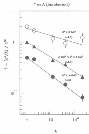
Fig. 5 The A dependence of the cross section for three Q^2 bins. The slopes change significantly as Q^2 rises.
