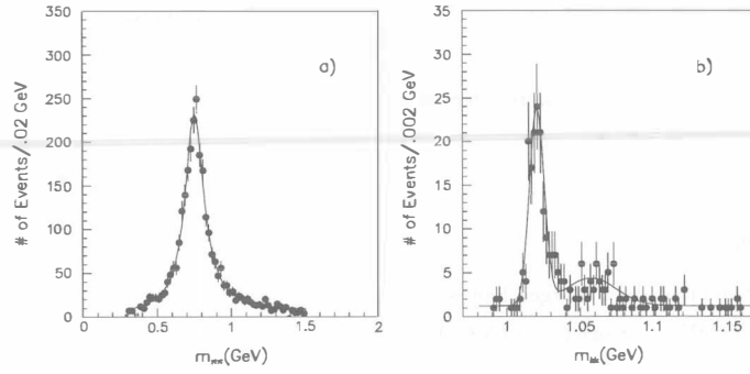
Fig. 2 The invariant masses for \pi\pi and KK pairs in the elastic peak.
