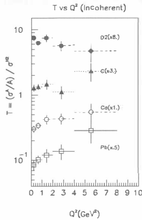
Fig. 4 The ratio of the elastic production cross sections/nucleon for deuterium, carbon, calcium and lead compared to hydrogen vs Q^2 .
