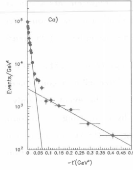
Fig. 3 The momentum transfer squared -t' = -(t - t_{min}) for the Calcium target, the spike at low -t' is due to coherent scattering from the entire nucleus.
