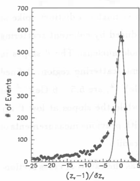
Fig. 1 The normalized elasticity, (z - 1)/\delta z , for all events in the \rho^0 or \phi mass regions. The curve is a gaussian fit to the data with z > 1 , the width is consistent with 1, as expected if \delta z is properly estimated.
