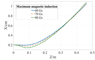
Figure 6: Envelope curves solved by transfer matrix with difference maximum magnetic fields in Z direction. Z starts from the entrance of the solenoid.
