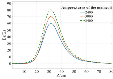
Figure 4: Magnetic field distributions as a function of the distance from the cathode. Lines of different colours represent different ampere turns of the solenoid.
