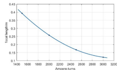
Figure 3: The focal length as a function of the NI number.
