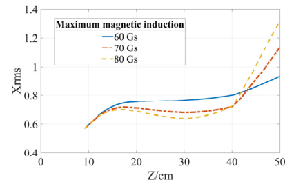
Figure 7: Envelope curves solved by PARMELA with difference maximum magnetic field in Z direction. Z starts from the entrance of the flange.
