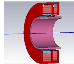
Figure 2: The 3D model of the solenoid lens.
