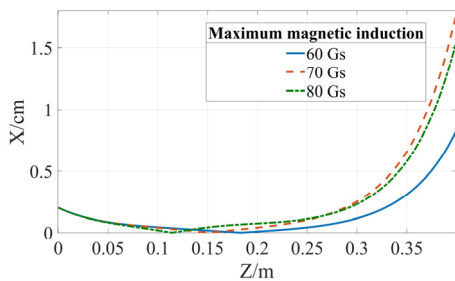
Figure 5: Envelope curves solved by K-V equation for the maximum magnetic induction in the Z direction on the solenoid axis for 80 Gs, 70 Gs and 60 Gs. Z starts from the entrance of the solenoid.
