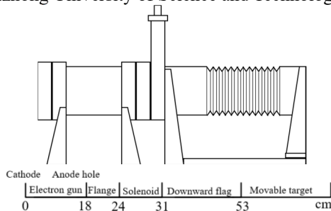
Figure 1: The layout of the compact beam diagnostics instrument built in HUST.
