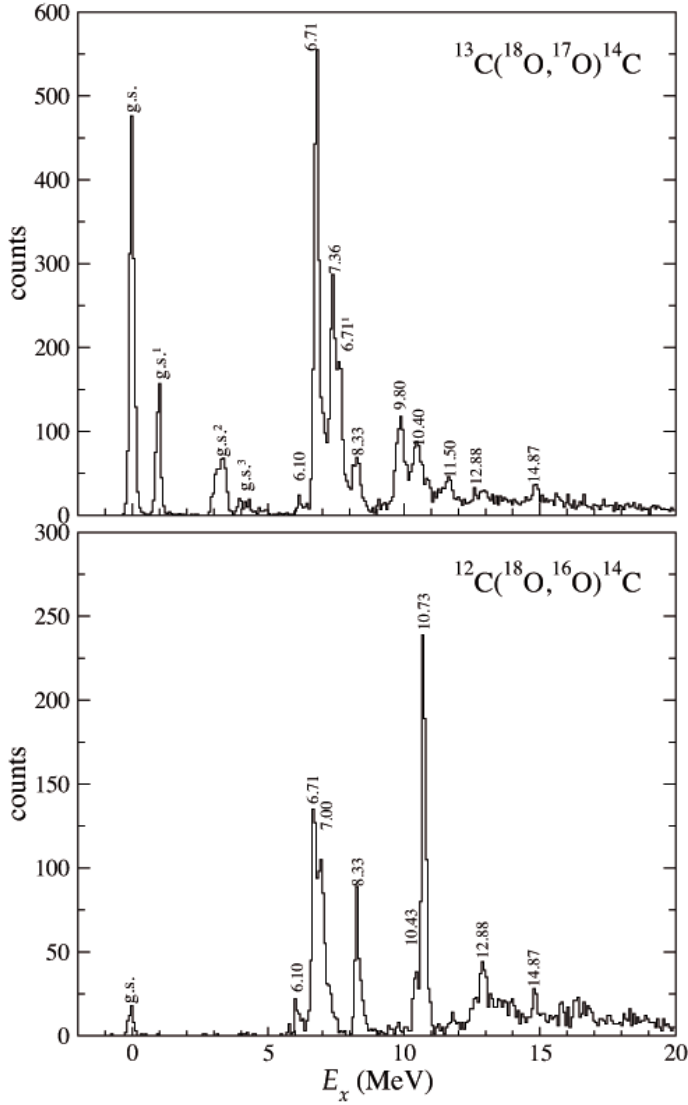
Fig. 1. ^{14}\text{C} energy spectra for the one- (top panel) and two- (bottom panel) neutron transfer for 4^\circ < \theta_{\text{lab}} < 5^\circ . In the top panel, the peaks marked with 1 , 2 , 3 represent the transition to the excited states of ^{17}\text{O} ejectiles at 0.87, 3.06, 3.84 MeV, respectively.
