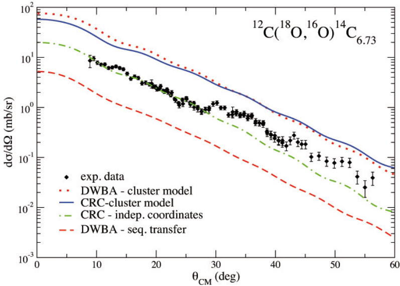
Fig. 2. (Color on-line) Comparison of the experimental angular distributions with theoretical calculations for the ^{12}\text{C}(^{18}\text{O}, ^{16}\text{O}) transition to the 6.73 excited state of the ^{14}\text{C} nucleus.
