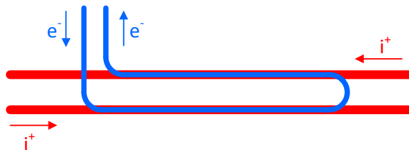
Figure 1: Scheme of cooling with one electron beam.
