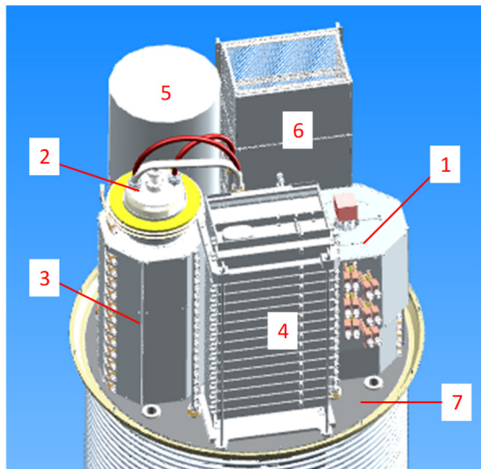
Figure 4: Scheme of cooling with one electron beam.
