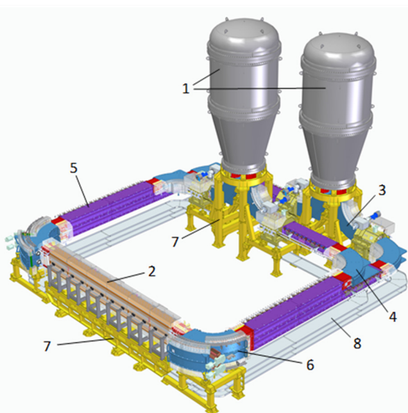
Figure 2: 3D model of the electron cooling system for NICA collider. 1 – high-voltage vessels, 2 – cooling section, 3 – vertical bend, 4 – horizontal bends, 5 – linear sections, 6 – toroid magnet, 7 – supports, 8 – cable channels.
