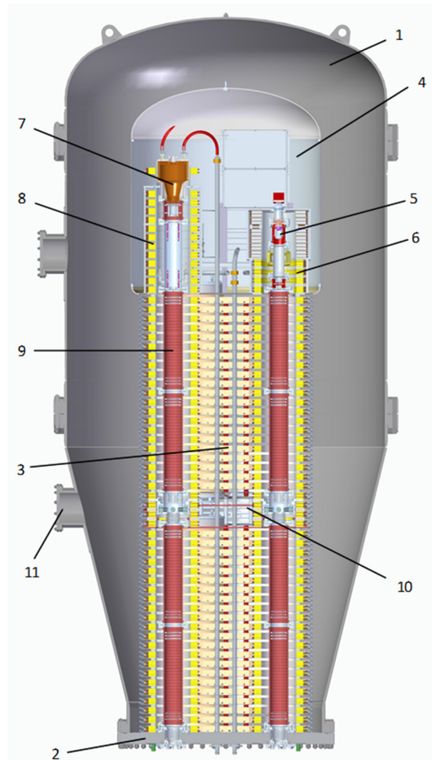
Figure 3: High voltage system of the electron cooler for NICA collider. 1 – pressure vessel, 2 – bottom flange, 3 – high voltage column, 4 – high voltage terminal, 5 – electron gun, 6 – gun solenoid, 7 – electron collector, 8 – collector solenoid, 9 – electrostatic tubes, 10 – middle section, 11 – side flange.
