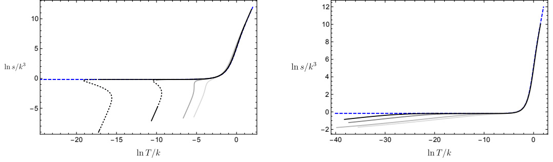
Figure 6.7: Plots of the entropy density s as a function of T for black hole solutions with various deformation parameters and for models with m^2 = -15/4 and \xi = -1/4 . The left plot is for \Gamma/k^{3/2} \leq \bar{\Gamma} \sim 19.37 , namely 5.5, 10.3, 18, and 19.3 (light grey to dark grey). The dashed blue line in both plots is for \Gamma/k^{3/2} = \bar{\Gamma} . For \Gamma/k^{3/2} = 19.33 and 19.36 we have used dotted lines on the curves to indicate the first order phase transition. As T \rightarrow 0 , for \Gamma/k^{3/2} < \bar{\Gamma} the black holes approach the boomerang RG flows, with s \sim T^3 , and when \Gamma/k^{3/2} = \bar{\Gamma} they approach the AdS_5^0 to AdS_2 \times \mathbb{R}^3 RG flow with, from (6.27), s \sim 0.84k^3 . The right plot is for \Gamma/k^{3/2} \geq \bar{\Gamma} , namely, 19.41, 19.75, 25 and 35 (dark grey to light grey). As T \rightarrow 0 the black holes have s \rightarrow 0 , but not as a power of T . At T \rightarrow 0 they approach insulating ground states. In both plots the intermediate scaling regimes can be seen.
