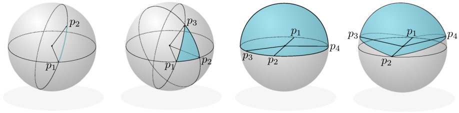
Fig. 3. The region S_R(u) in the cases N = 2, 3, 4
