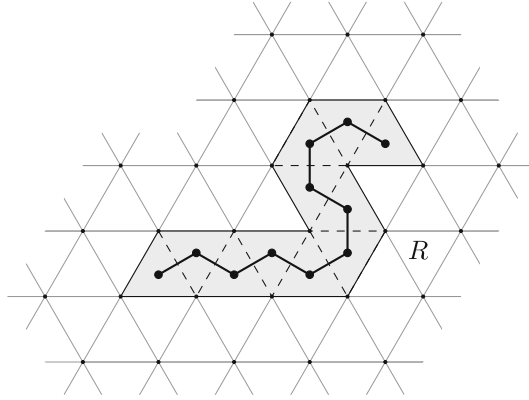
Fig. 2. Construction of the planar graph in the proof of Lemma 5.1 (same notation as in Fig. 1)
