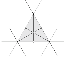
Fig. 5. Subdivision of an elementary cell of \mathcal{L}_\varepsilon into cells of \mathcal{L}'_\varepsilon . The points of \mathcal{L}^m_\varepsilon are indicated in white, while those in \mathcal{L}^c_\varepsilon are indicated in gray
