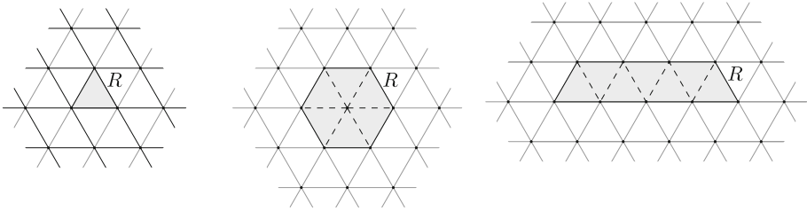
Fig. 1. Examples of the different possible interpolation regions R according to Lemma 5.1. The dashed and the continuous lines denote edges in \mathcal{N}_\varepsilon(u) and \mathcal{C}_\varepsilon(u) , respectively
