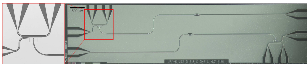
Figure 3. Microscope picture of the chip comprising two JPA devices. Each JPA device consist of an aluminum resonator terminated with a dc-SQUID, a pump transmission line and a dc-flux line.
