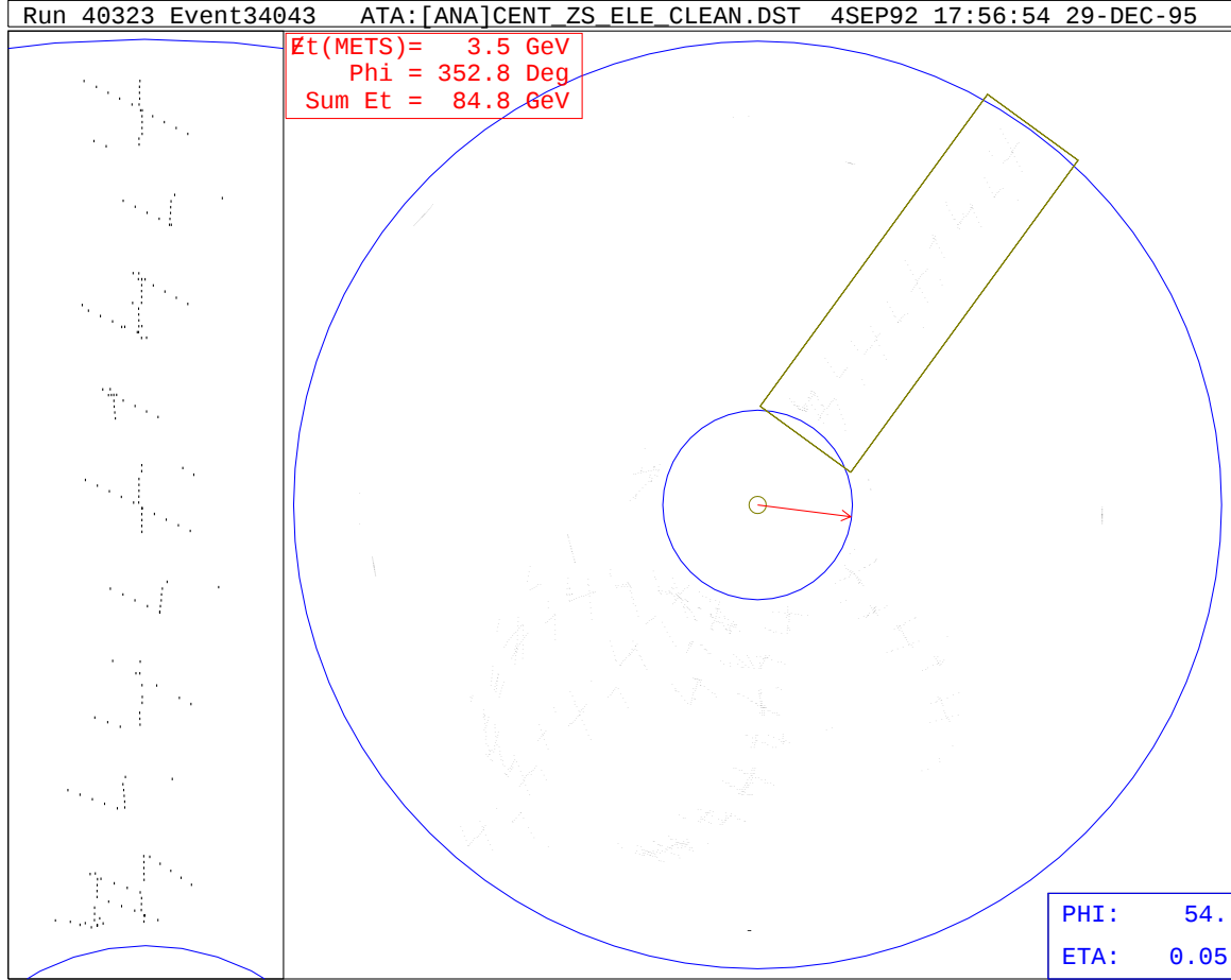
Figure 4-4: Display of CTC information for a Z^0 \rightarrow e^+e^- candidate from 1992. The display on the left is an expansion of the indicated region in the display on the right. Dots indicate the locations of the recorded hits; both real and ghost hits are shown. The large angle between the real and ghost stubs for the high p_T tracks makes it simple to differentiate between them. The hit information assumes z = 0 , so the points on the stereo layers do not line up exactly with those on the axial layers.
