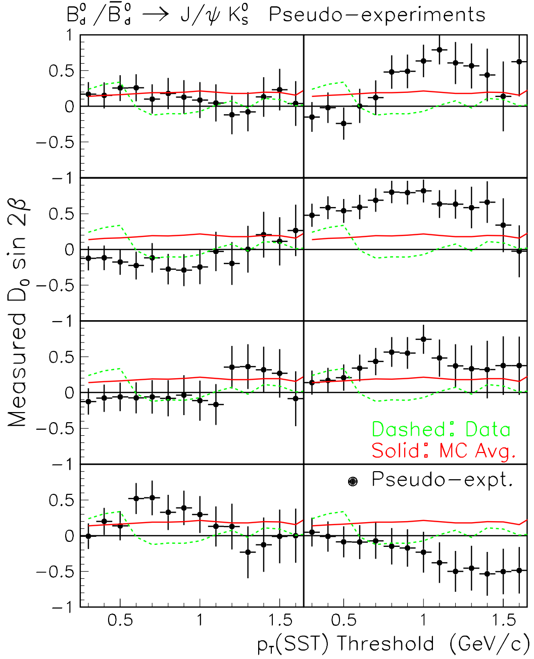
Figure 11-6: The variation of \mathcal{D}_0 \sin 2\beta with the p_T(\text{SST}) cutoff for the first eight J/\psi K_S^0 Monte Carlo subsamples. The solid curve indicates the average Monte Carlo values, and the dashed curve indicates the results from the data. The points are the results from individual Monte Carlo subsamples.
