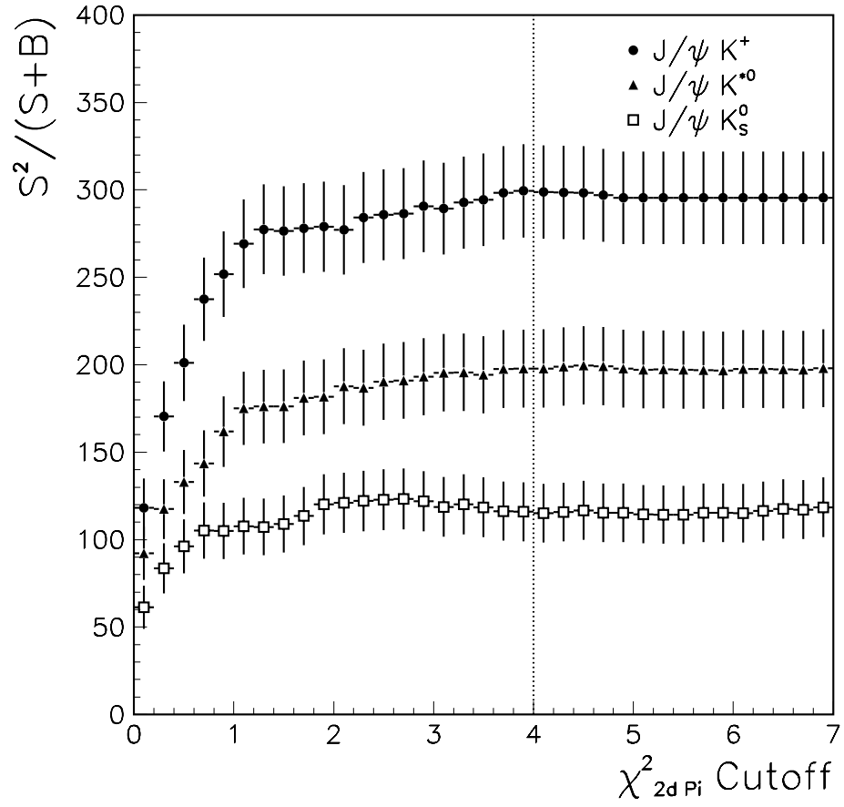
Figure 6-5: Dependence of S^2/(S+B) on the \chi^2_{2d\text{ pi}} cutoff. The vertical line shows the cutoff used in this analysis: candidates with \chi^2_{2d\text{ tr}} > 4 are rejected.
