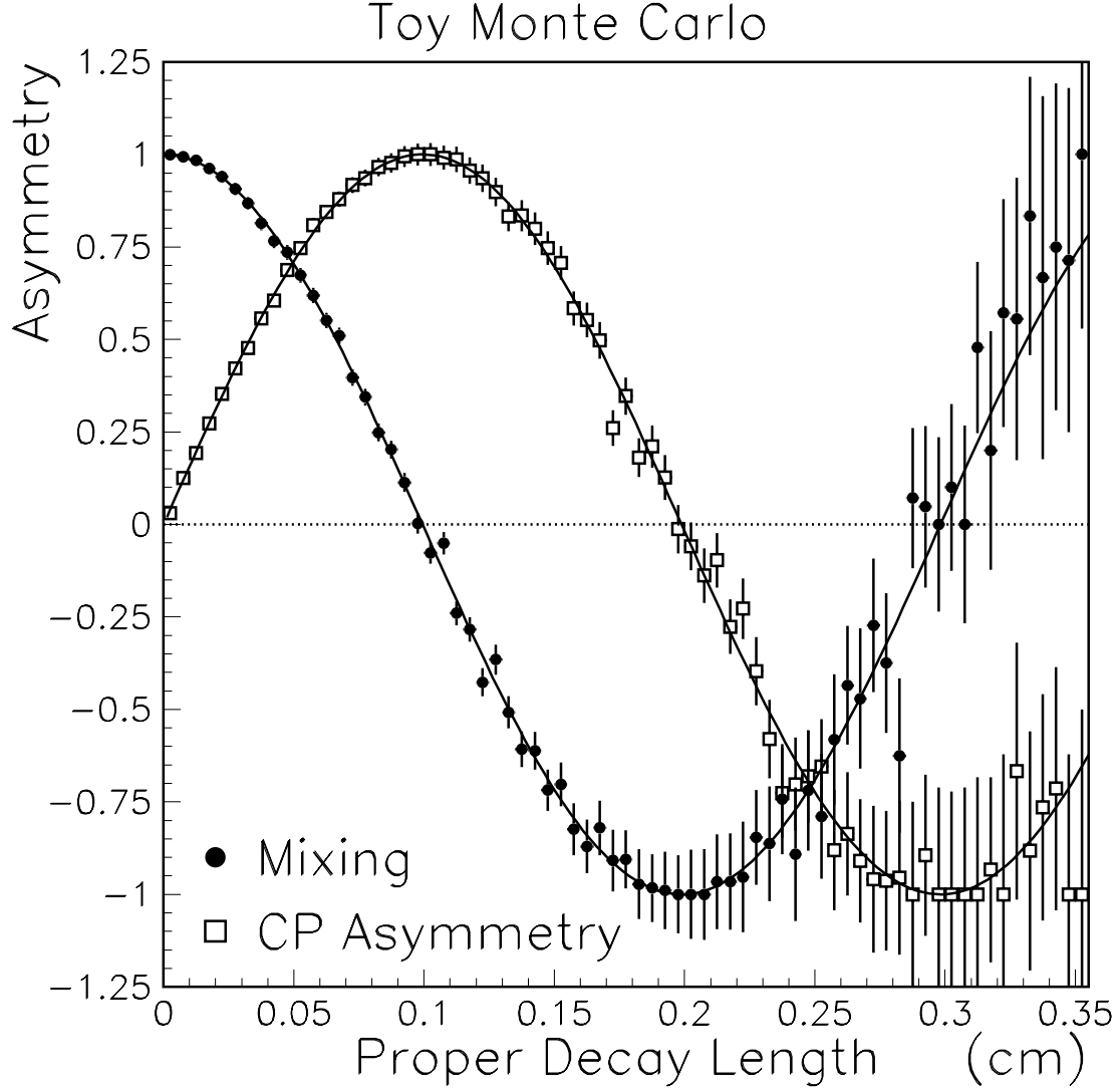
Figure B-2: Asymmetries in the Toy Monte Carlo. The mixing asymmetry is in the number of unmixed versus mixed signal events in J/\psi K^{*0} . The CP asymmetry is the in the number of \bar{B}^0 versus B^0 in J/\psi K_S^0 . The horizontal scale is the “true” (unsmeared) decay length. The curves indicate the expected asymmetries. The statistics are several hundred times higher than those in the data.
