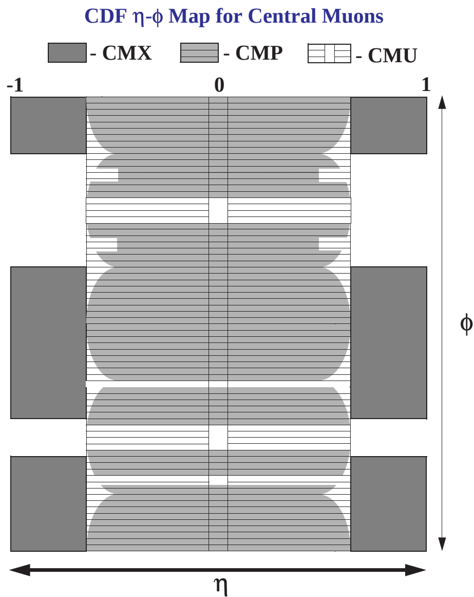
Figure 4-7: Regions of \eta - \phi space covered by the CMU, CMP, and CMX.
