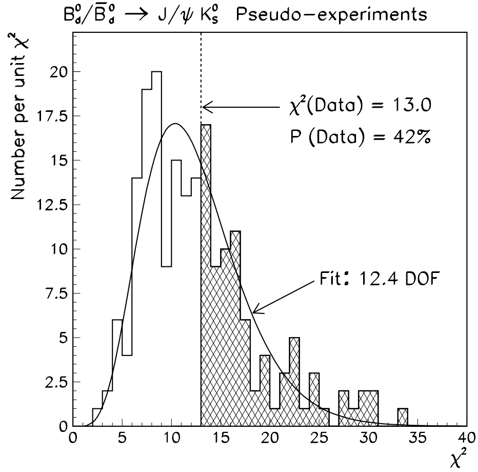
Figure 11-10: The distribution of \chi^2 returned by the J/\psi K_S^0 Monte Carlo samples. The fit is to f(z; n) = z^{n/2-1} e^{-z/2} / 2^{n/2}, (n/2) , which corresponds to the standard \chi^2 with n degrees of freedom.
