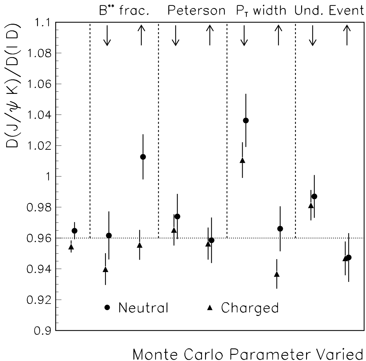
Figure 12-8: Ratio of dilution for low p_T B mesons to that of high p_T B mesons. The horizontal scale indicates which Monte Carlo sample is being compared to the nominal Monte Carlo sample. Uncertainties are due to MC statistics. Zero is suppressed on the vertical scale.
