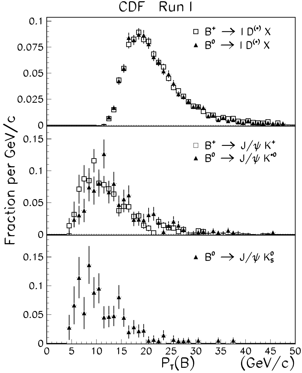
Figure 12-1: Distributions of p_T(B) for the J/\psi K and \ell-D data.
