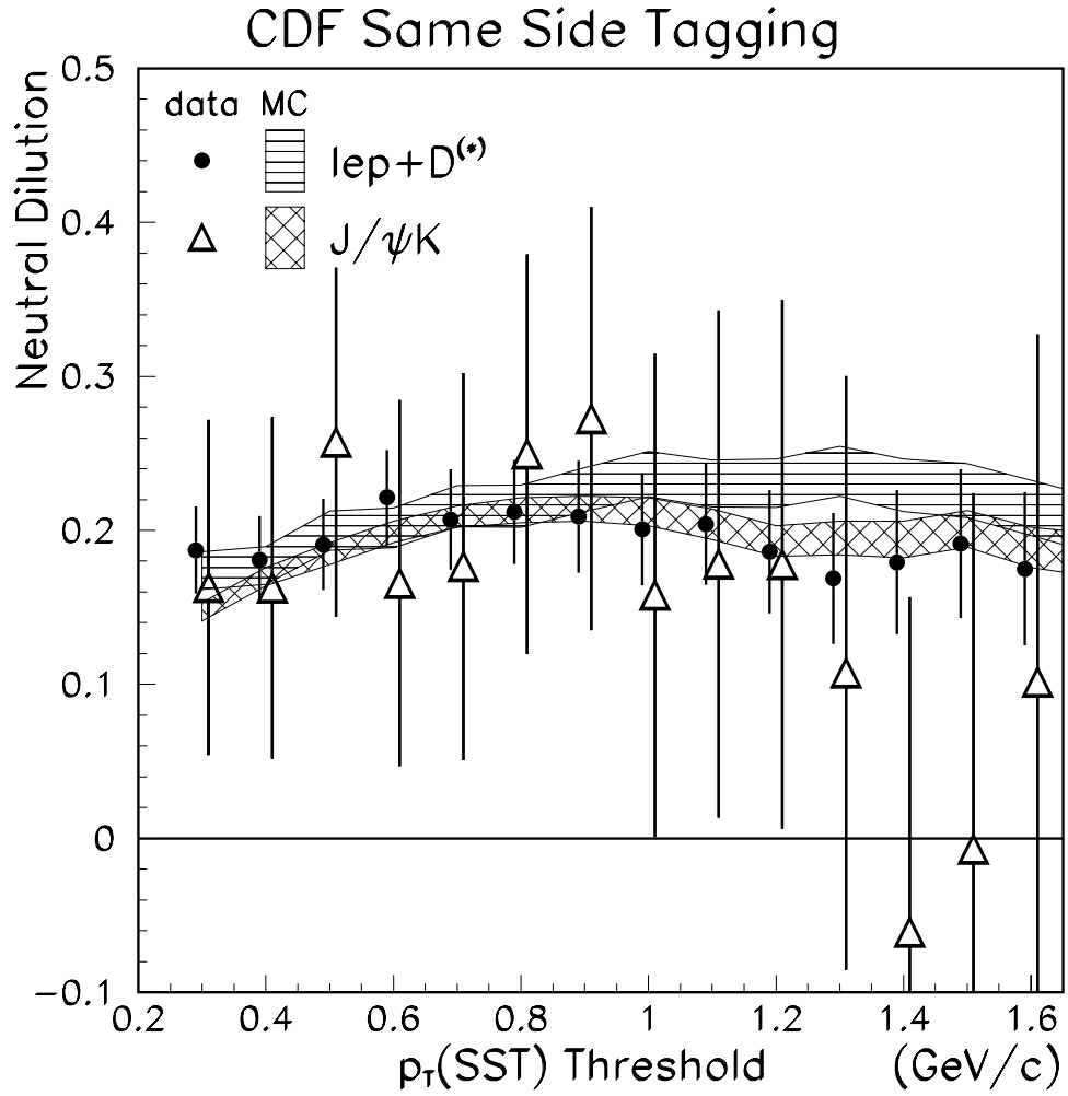
Figure 11-4: The variation of \mathcal{D}_0 with the p_T(\text{SST}) cutoff for J/\psi K and \ell\text{-}D data and Monte Carlo. The points for each sample are partially correlated with one another, so it is not possible to judge the expected point-to-point variation from the information given.
