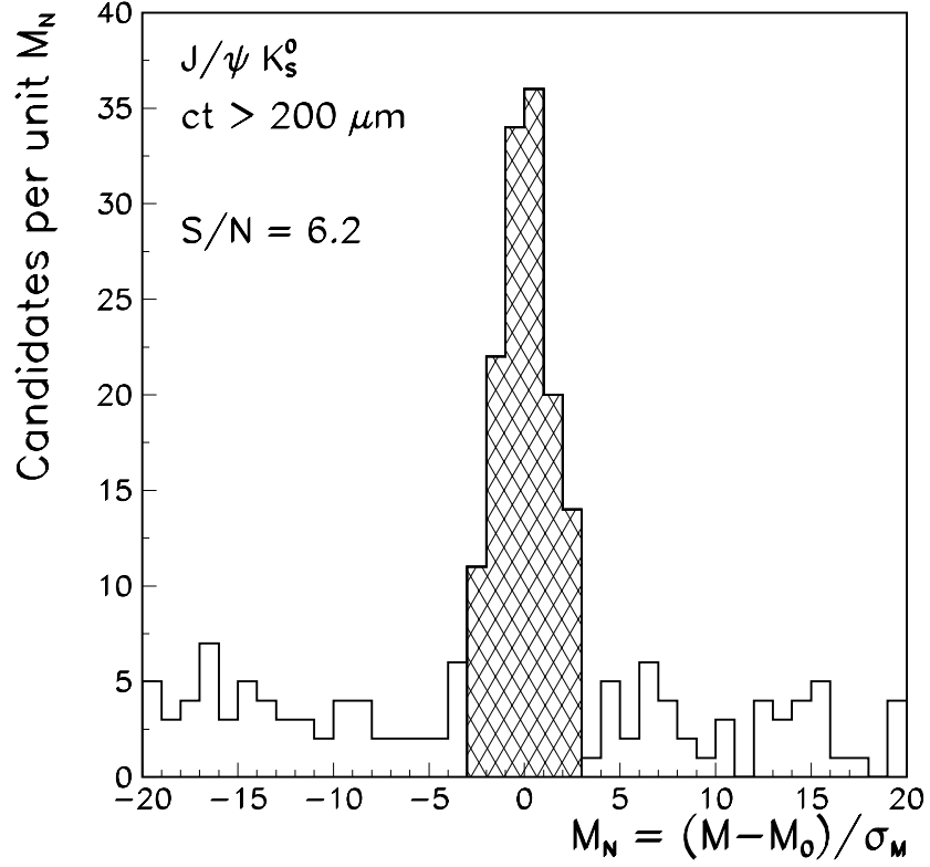
Figure 10-10: Normalized mass distribution for J/\psi K_S^0 events with ct > 200 \mu\text{m} . There are 137 events with |M_N| < 3 , of which 19 are estimated to be background and are \sim 118 estimated to be signal. The ratio of signal to background is S/N = 6.2 .
