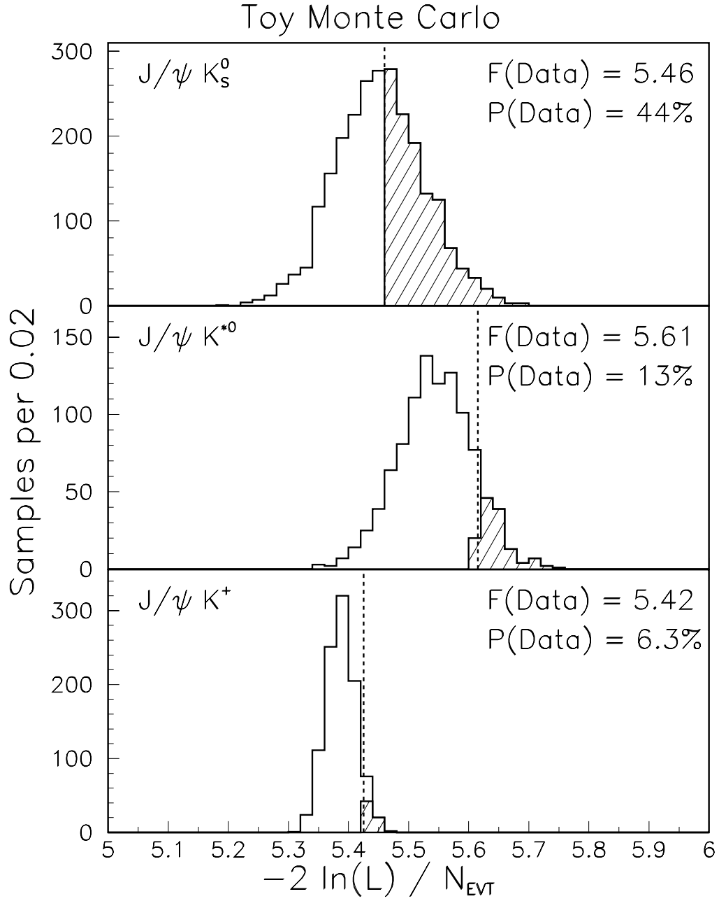
Figure B-5: Distributions of F \equiv -2 \ln(\mathcal{L}) / N_{\text{evt}} for the J/\psi K_S^0 , J/\psi K^{*0} , and J/\psi K^+ Toy Monte Carlo samples. The vertical dashed lines indicate the values of F for the data, and the hashed histograms indicate the TMC samples which have F larger than that in the data.
