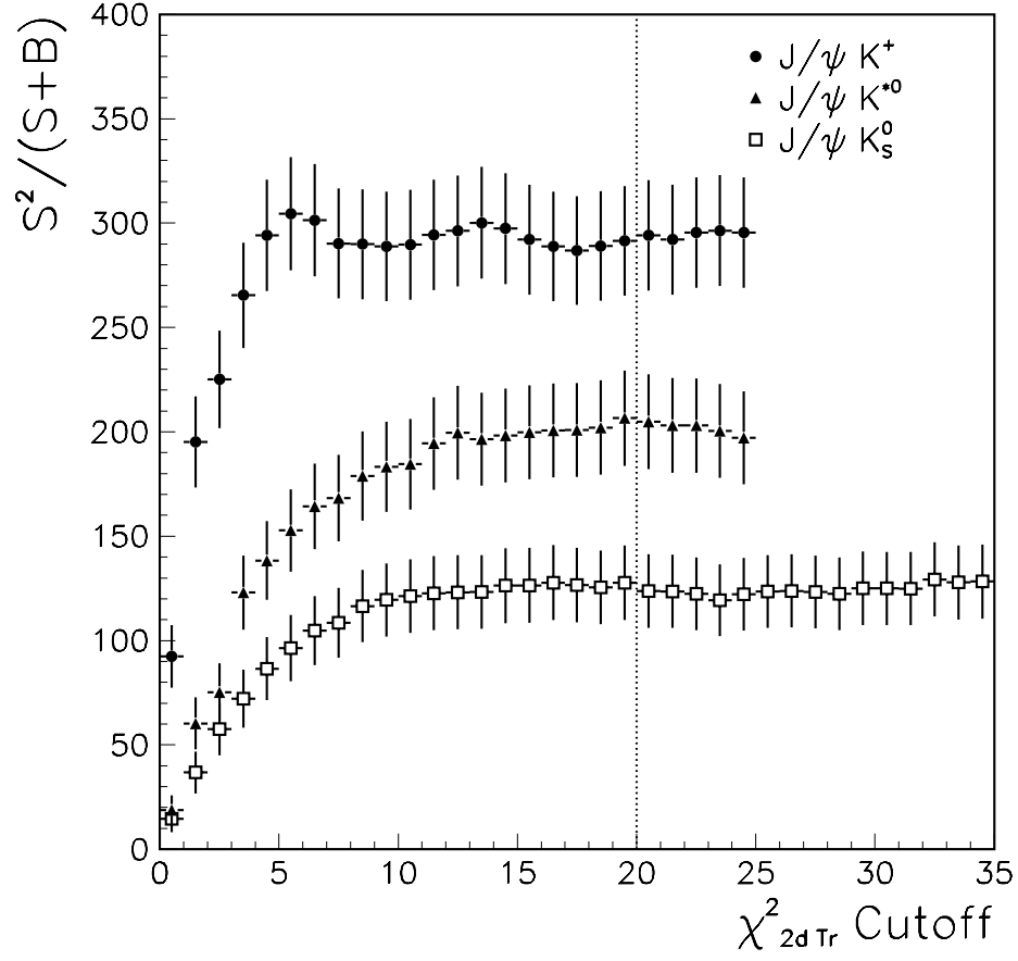
Figure 6-4: Dependence of S^2/(S+B) on the \chi^2_{2d\text{tr}} cutoff. The vertical line shows the cutoff used in this analysis: candidates with \chi^2_{2d\text{tr}} > 20 are rejected. This information was not collected for J/\psi K^+ or J/\psi K^{*0} candidates for cutoffs above 25.
