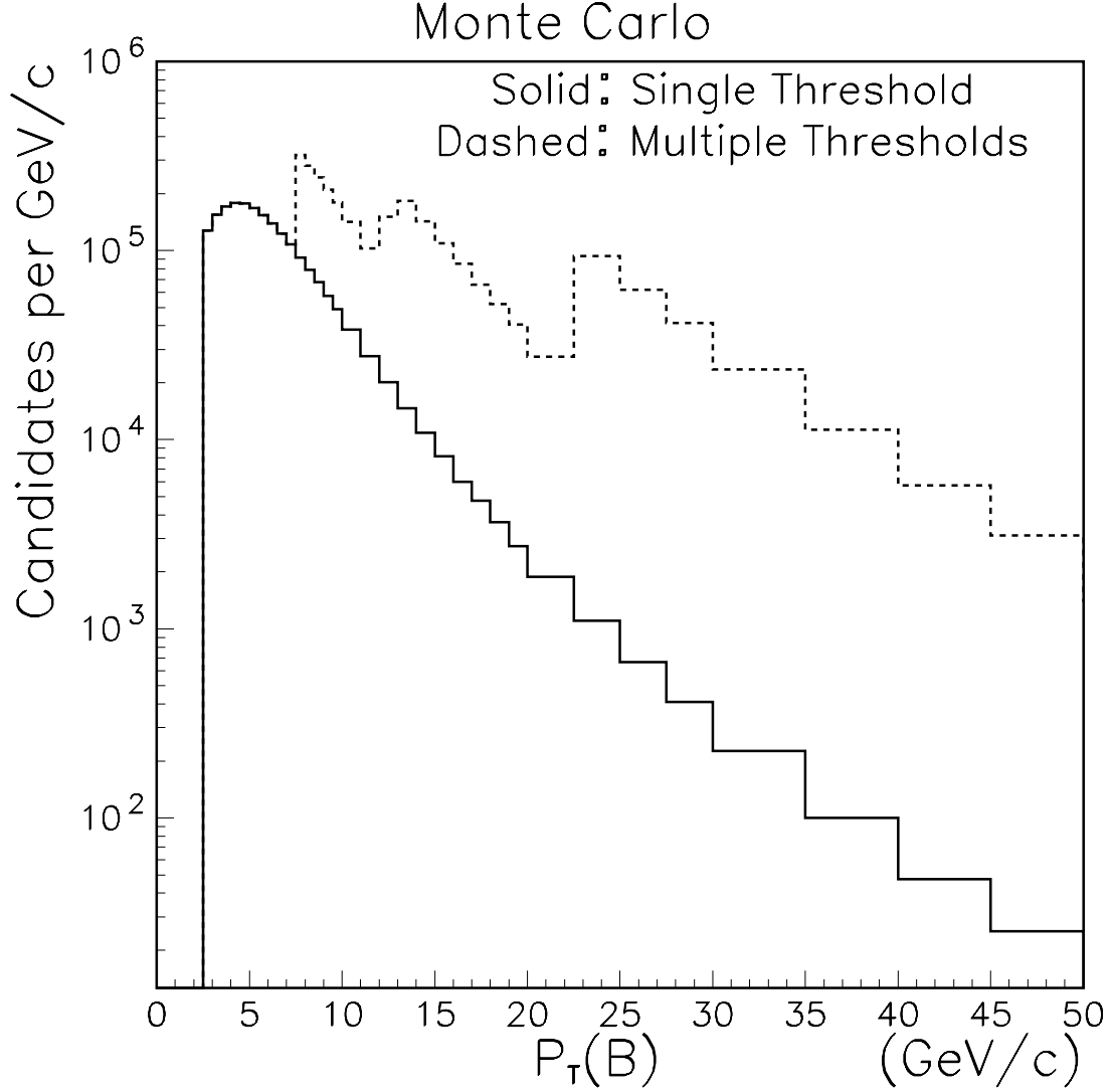
Figure A-1: p_T distribution for generated B mesons. The histogram is normalized by bin-width, so the vertical scale is “Candidates per GeV/ c ,” for all bins, despite varying bin sizes. The solid histogram is for the sample generated with p_T(b) threshold of 0. The dashed histogram also includes the other three samples, which are generated with thresholds of 5, 10, and 20 GeV/ c .
