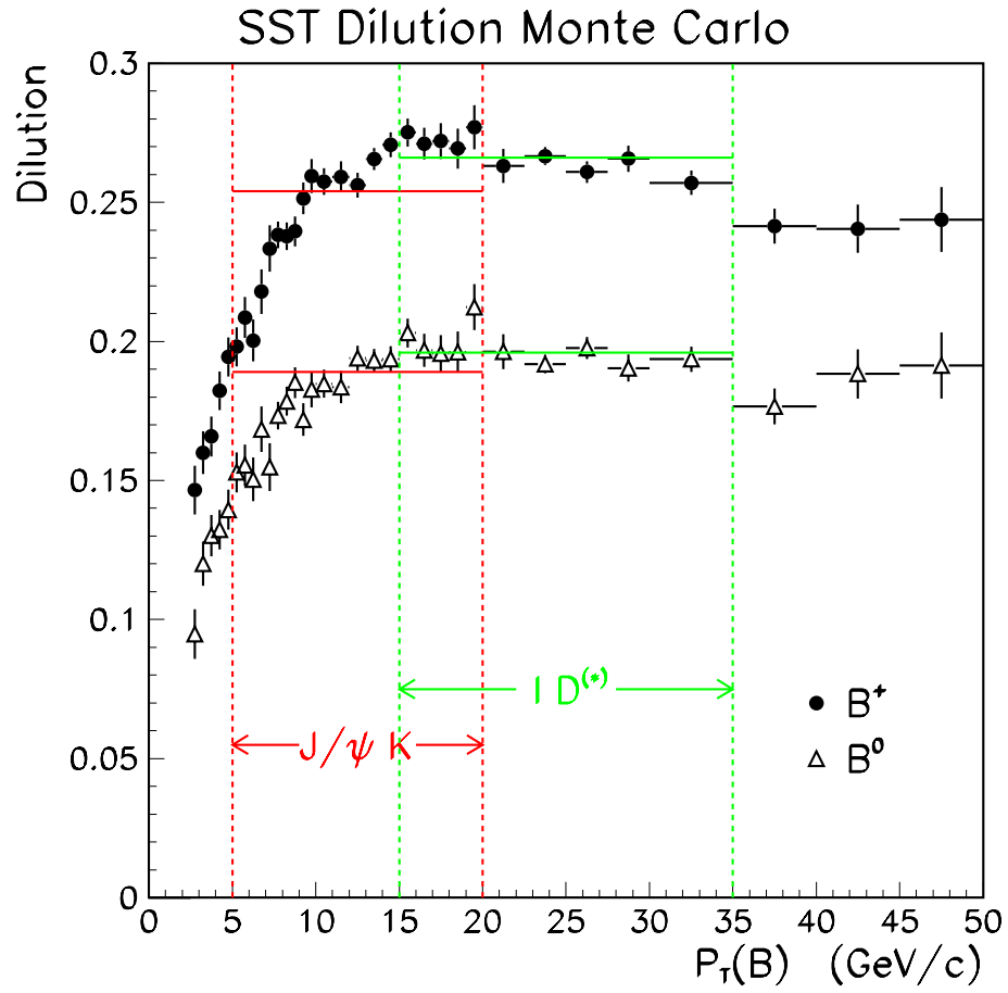
Figure 12-3: Dilution vs p_T(B) for MC. The vertical bands indicate typical p_T(B) regions for the J/\psi K and \ell-D samples. The horizontal lines indicated the Monte Carlo predicted dilutions for the J/\psi K and \ell-D samples (below).
