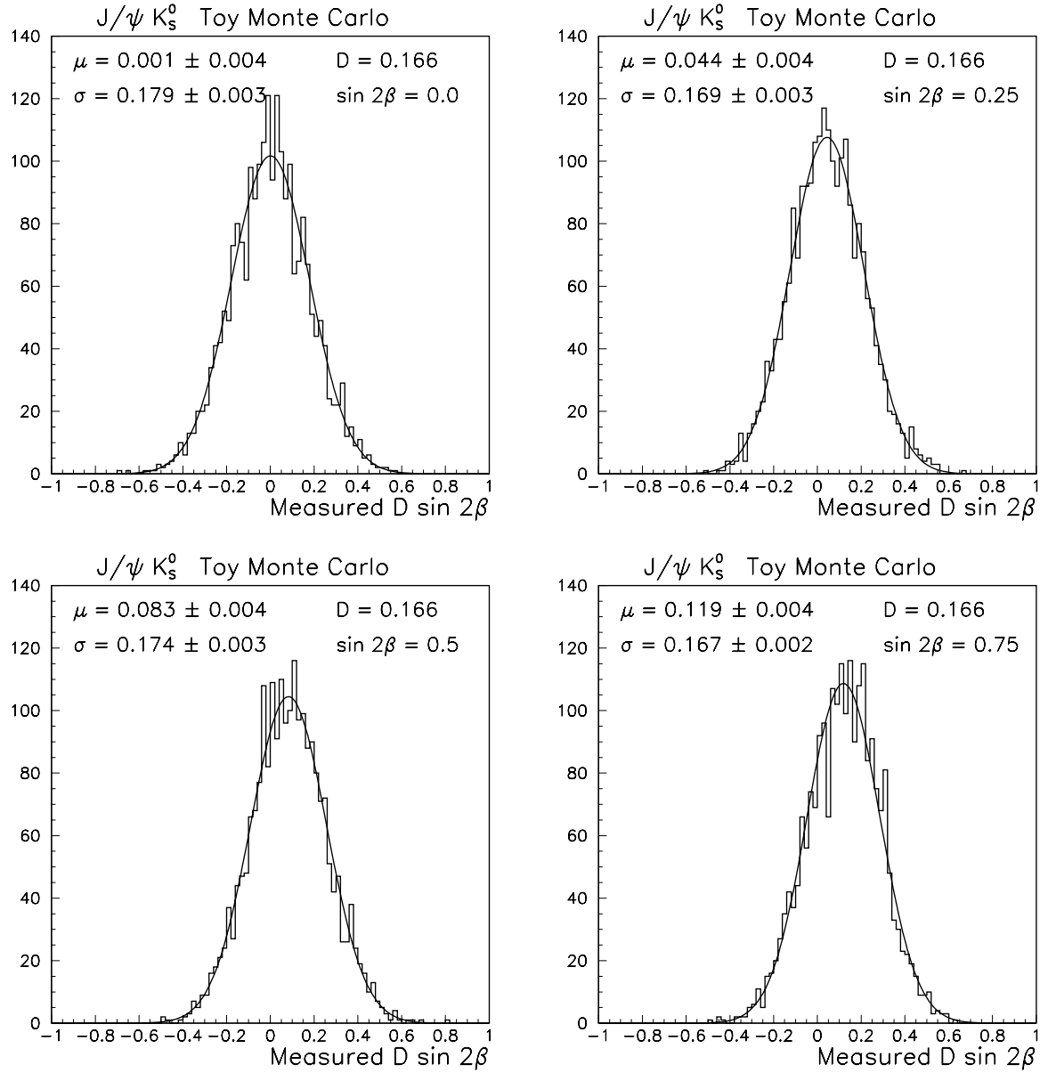
Figure B-4: Distributions of raw CP asymmetries fit for in TMC samples with varying input values for \sin 2\beta . The top-left plot is generated with \sin 2\beta = 0 , top-right with \sin 2\beta = 0.25 , bottom-left with \sin 2\beta = 0.5 , and bottom-right with \sin 2\beta = 0.75 . The curves represent Gaussian fits to the distributions, with the indicated mean ( \mu ) and width ( \sigma ). Each mean is consistent with the respective value of D \sin 2\beta .
