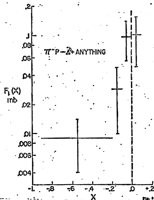
Fig. 4. Inclusive \bar{\Lambda} production in 205 GeV/c \pi^-p interactions.
