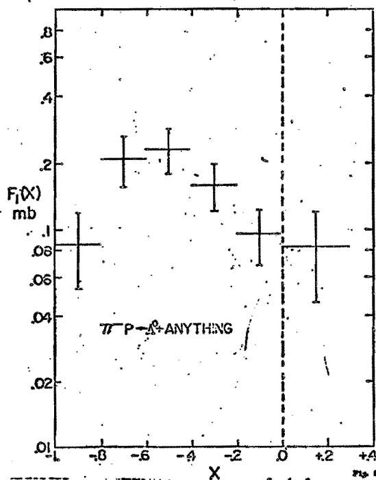
Fig. 3 Inclusive \Lambda production in 205 GeV/c \pi^-p interactions.
