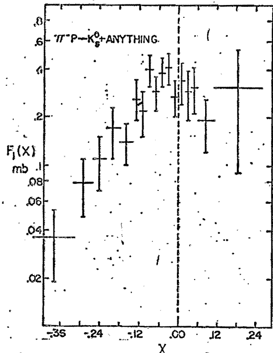
Fig. 2 Inclusive K_S^0 production in 205 GeV/c \pi^-p interactions.
