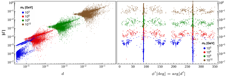
Fig. 2. (Color online) Scatter plot of the parameters d , |d'| , and \phi' . \tilde{m}_2 = 8.7 \text{ meV} and \tilde{m}_3 = 49.6 \text{ meV} are calculated from Eq. (34) with the \Delta m^2 taken from [5]. For \tilde{m}_4 , we assume the values \{10^3, 10^6, 10^9, 10^{12}\} \text{ GeV} and m_D^2 = 0.81 \tilde{m}_3 \tilde{m}_4 . The parameters of the Higgs sector are taken from [6].
