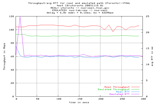
Figure 4: Comparison of an emulation and the real path measurements.
