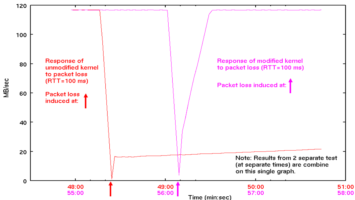
Figure 6: Throughput in modified and unmodified Linux kernel achieved in the emulator.
