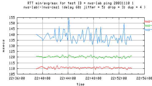
Figure 2: Example of emulated delay and jitter
