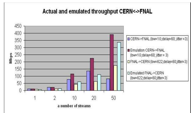
Figure 6: GridFTP in emulation and in the real path.
