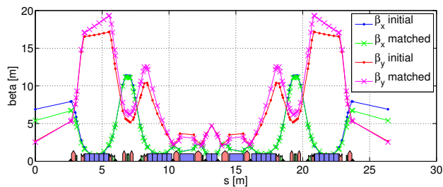
Figure 3: Varying of the \beta functions using atmatch .
