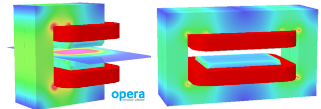
Figure 2: Possible C-type (left) and H-type (right) dipole magnet designs. The magnetic field strength within the magnet is indicated by colour map. For the C-type magnet, the magnetic field on axis is also illustrated
