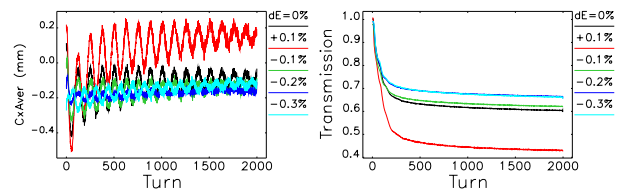
Figure 4: Left: Average horizontal beam position for different booster extraction energy. Right: Beam transmission for different booster extraction energy.
