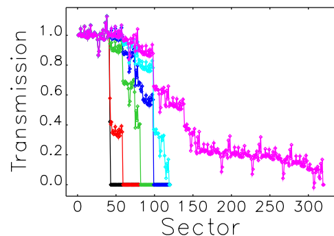
Figure 2: Beam transmission improvement by equalizing the coordinates at the end of sector 40 to the coordinates of the injected beam. Several iterations are shown, one turn equals 40 sectors.
