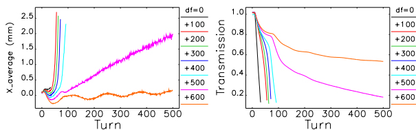
Figure 3: Average horizontal beam position (left) and beam transmission (right) as a function of turns for different rf frequency.
