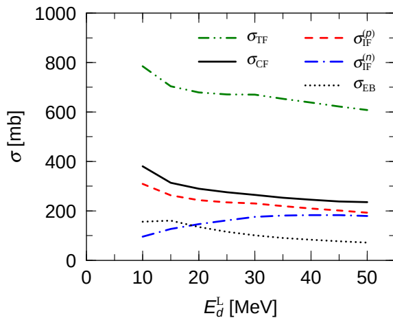
Figure 8. Results of the total fusion cross section \sigma_{\text{TF}} (dash-double-dotted line), complete fusion cross section \sigma_{\text{CF}} (solid line), proton-absorbed cross section \sigma_{\text{IF}}^{(p)} (dashed line) and neutron-absorbed cross section \sigma_{\text{IF}}^{(n)} (dash-dotted line) for the deuteron induced reaction on {}^7\text{Li} as a function of the deuteron incident energy E_d^L . The dotted line represents the elastic breakup cross sections calculated with CDCC.
