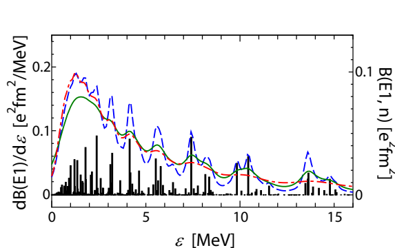
Figure 2. E1 strength distribution of {}^6\text{He} as a function of \epsilon . The bars show B(E1; n) from the 0^+ ground state to the n th pseudostates of {}^6\text{He} . The solid, dashed and dash-dotted lines respectively show the smeared E1 strength distributions assuming the Lorentzian form with the width of 0.5, 0.2 and 0.1(\epsilon_n + 0.975) MeV; \epsilon_n denotes the eigenenergy of the n th pseudostate.
