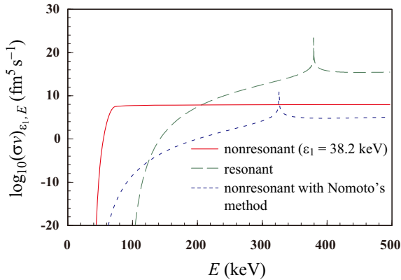
Figure 7. The solid and dashed lines show the reaction probability (\sigma v)_{\epsilon_1, E} for the nonresonant ( \epsilon_1 = 38.2 keV) and resonant processes, respectively. The dotted line shows the result for the nonresonant process with Nomoto's approximation in CDCC calculation.
