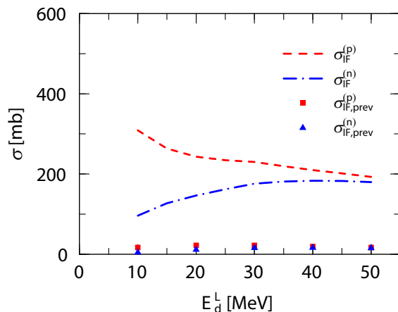
Figure 9. \sigma_{\text{IF}}^{(p)} (dashed line) and \sigma_{\text{IF}}^{(n)} (dash-dotted line) calculated with the present method, compared with \sigma_{\text{IF,prev}}^{(p)} (squares) and \sigma_{\text{IF,prev}}^{(n)} (triangles) following the previous definition given in Refs. [42] and [43].
