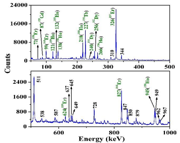
Fig. 1: Gamma ray spectrum obtained with irradiated ^{159}\text{Tb} target
