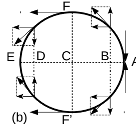
FIG. 2: Various positions of the paired valence neutrons in ^{11}\text{Li} , at point A the c.m. of the two neutrons is at rest with respect to ^9\text{Li} but the relative momenta of the neutrons is largest. At this position it is difficult to remove a single neutron because of their close proximity hence the two neutron removal results in the narrow momentum component.
