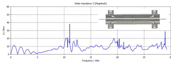
Figure 5: Longitudinal beam impedance of single kicker section simulated with CST Microwave Studio®.
