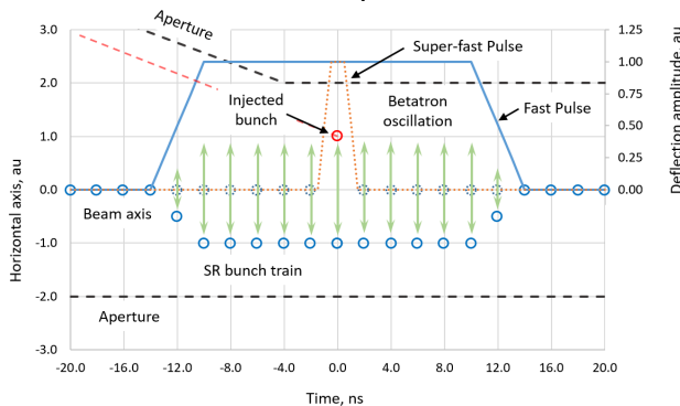
Figure 1: Simplified representation of “Fast” and “Super-fast” injection in “aperture sharing” mode.
