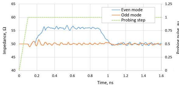
Figure 4: Even and odd mode TDR of one kicker section, probing step rise time 100 ps simulated with CST Microwave Studio®.
