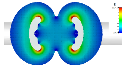
Figure 3: Kicker blades cross section with indicated relative surface electric field.
