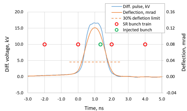
Figure 7: Differential voltage pulse waveform of FID GmbH pulse generator and the numerically calculated one kicker section deflection (in electron bunch frame).
