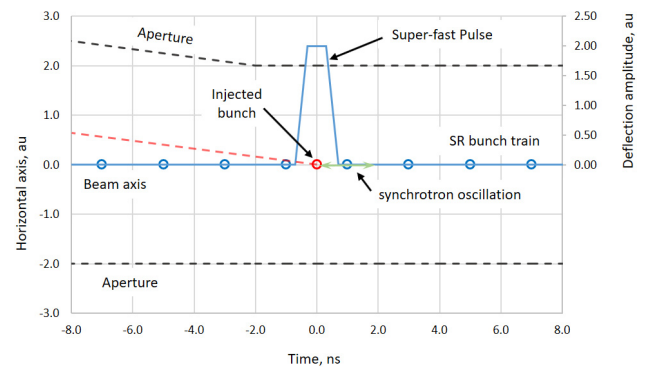
Figure 2: Simplified representation of “on-axis” injection mode with “Super-fast” scheme.
