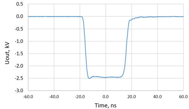
Figure 6: Output pulse waveform of 5-stage prototype GaN JFET based Marx generator.
