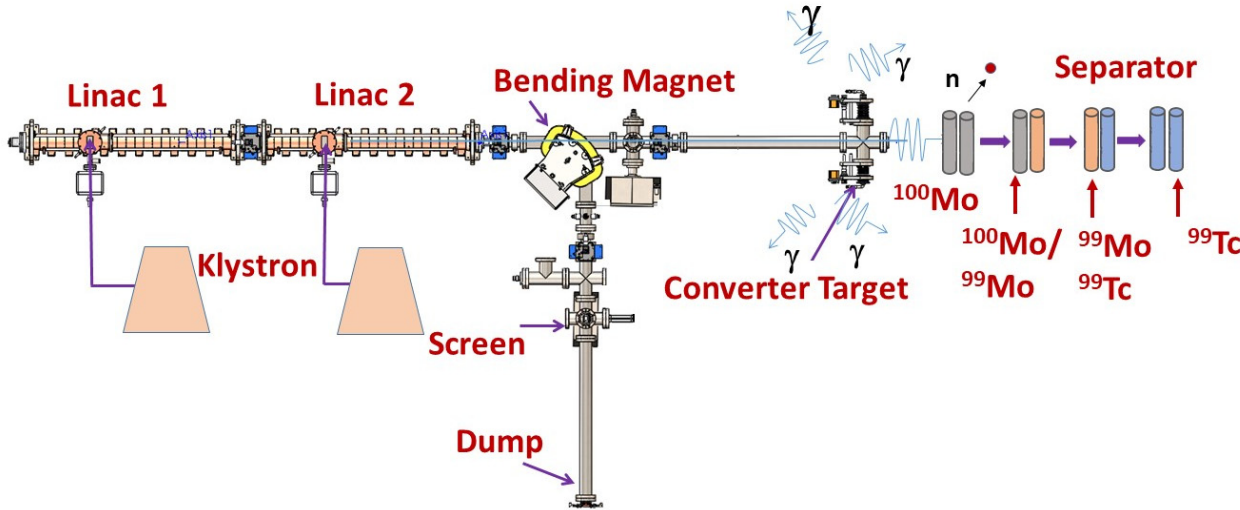
Figure 2: Schematic of SAMEER Linac based system for isotope generation.
