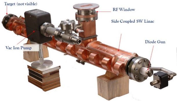
Figure 3: SAMEER side coupled structure.
