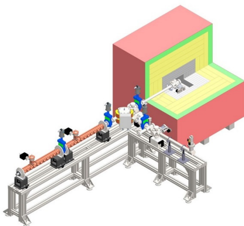
Figure 4: System with local shielding structure.
