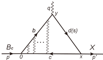
Fig. 3. Ladder Feynman diagram of the Coulomb-like correction.
