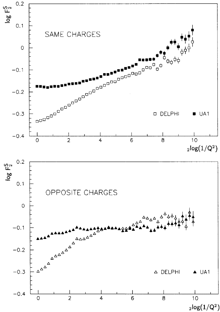
Fig. 6.2. Comparison of density integrals for q = 2 in their differential form \Delta F_2 (in intervals Q^2, Q^2 + dQ^2 ) as a function of 2\log(1/Q^2) for e^+e^- (DELPHI) and hadron-hadron collisions (UA1). [166]
