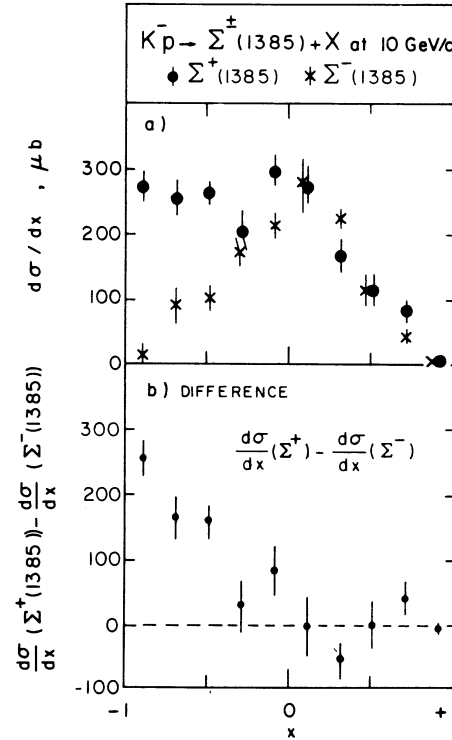
Fig. 1.9. (a) Differential cross section d\sigma/dx for \Sigma^+(1385) and \Sigma^-(1385) inclusive production at 10 GeV/c. (b) Difference between the d\sigma/dx distribution for \Sigma^+(1385) and that for \Sigma^-(1385) [56].
