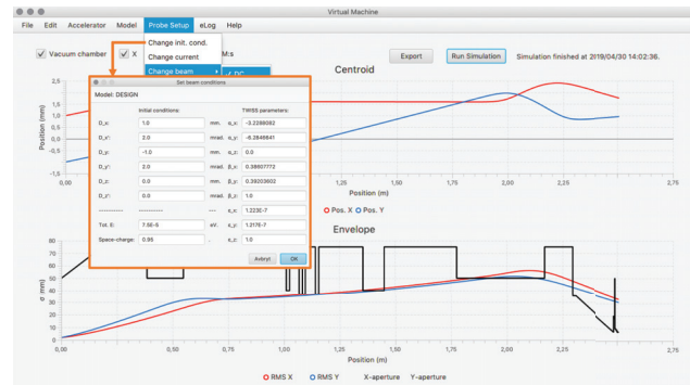
Figure 3: The new OpenXAL VM GUI with the ESS LEPT set up. Functionalities shown are the setting up a beam for simulation and the plots of the simulated DC beam's centroid and envelope functions.
