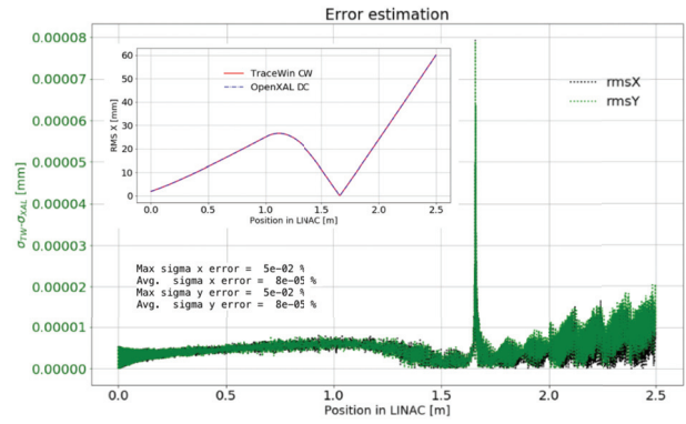
Figure 1: Simulation of a 10 mA DC beam through a hard-edge solenoid magnet. The main figure shows the absolute value of the difference between the beam envelope results from TraceWin and OpenXAL, whilst the inset shows the absolute values of the horizontal beam envelope.
