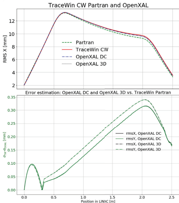
Figure 2: Beam simulation of a 74 mA DC beam through the LEPT section of the ESS proton Linac. The top figure shows the horizontal beam envelope (RMS beam sizes) for the simulations, whilst the bottom figure shows the difference between the beam envelope results from the two OpenXAL beam models and the TraceWin results with Partran.
