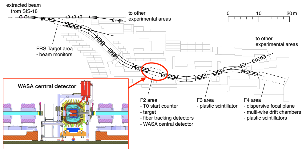
Fragment Separator at GSI
