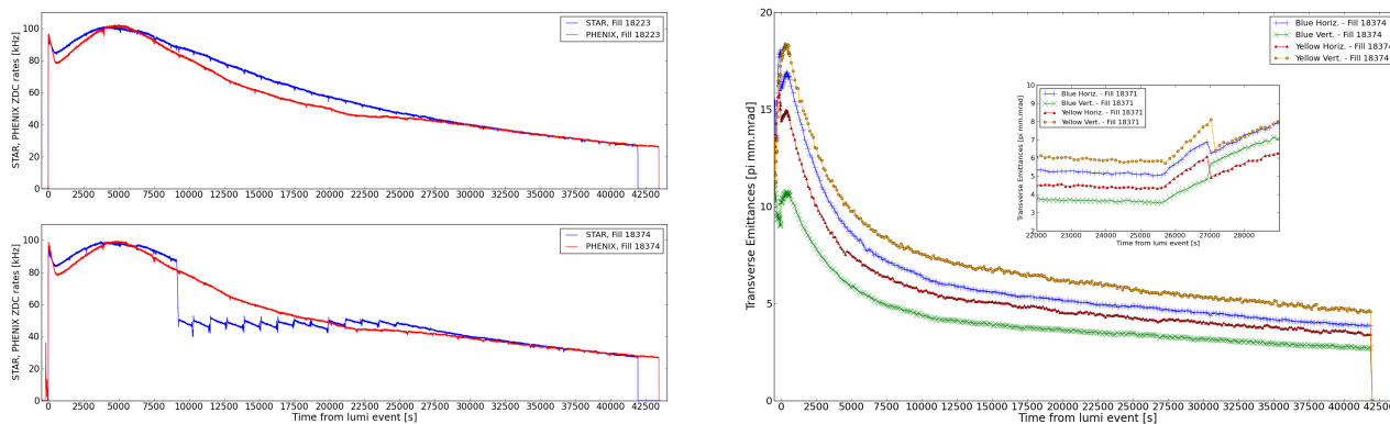
Figure 2: Left : collision rates (ZDC) for the STAR and PHENIX experiments for the two best 100 GeV Au-Au fills in regular (top) and target (bottom) mode. For the latter, the STAR ZDC rates are dropped to 50 kHz 3 hours (later re-optimized to 2.5 hours) into each store to maximize the integrated luminosity delivered to the HFT. - Right : horizontal and vertical transverse emittances of the Blue and Yellow beams for a typical RHIC 100 GeV Au-Au store with stochastic cooling on (main) and turned off at the end of a store (inclusion) during a dynamic \beta^* squeeze experiment.
