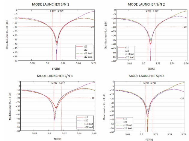
Figure 4: Reflection characteristics measured for the four fabricated mode launchers.
