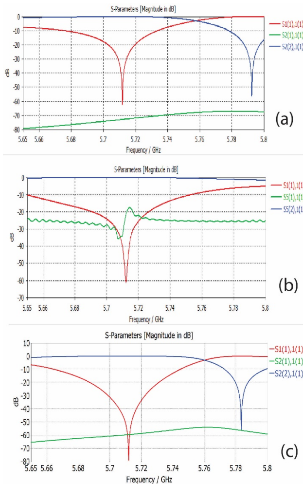
Figure 2: CST Microwave Studio simulations of S-parameters in various designs of the mode launchers: (a) LANL's design; (b) INFN's design scaled to C-band; (c) UCLA's design scaled to C-band.
