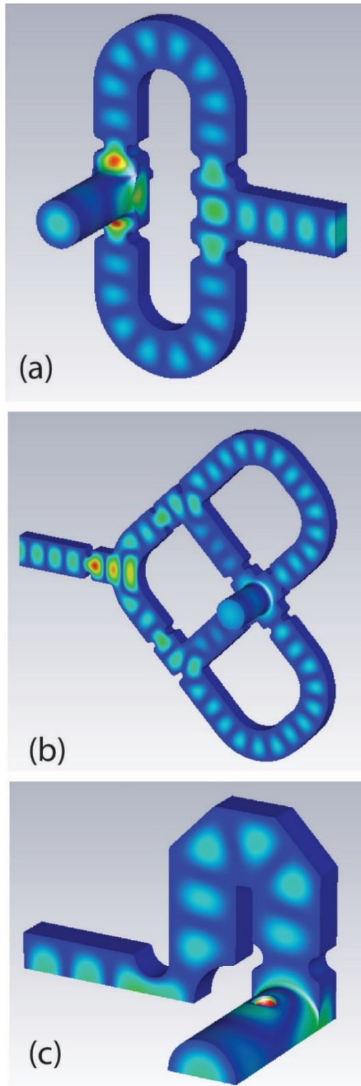
Figure 1: CST Microwave Studio simulations of the electric field magnitude in various designs of the mode launchers: (a) LANL's design; (b) INFN's design scaled to C-band; (c) UCLA's design scaled to C-band. For UCLA's design only a half of the whole mode launcher is shown and the perfect-H boundary condition is used at the bottom plane.
