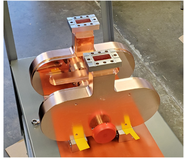
Figure 3: A photograph of two mode launchers fabricated by Dymenso, LLC.
