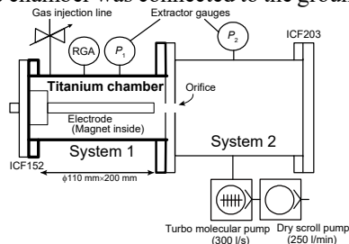
Figure 6: Setup for examining the surface oxide film removal by the sputtering. System 1 and 2 are connected with the orifice. Only system 2 is evacuated by the TMP.
