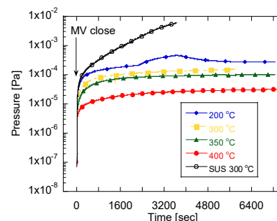
Figure 4: Build-up result of the total pressure after baking at each temperature. The result for the SUS chamber baked at 300 °C is also shown for comparison.
