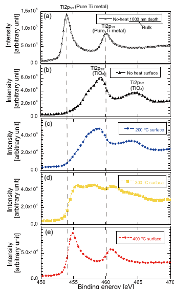
Figure 2: Photoelectron spectra of Ti2p . a) Bulk of the unbaked sample. b) Surface of the unbaked sample. c-e) Surface of the baked sample at 200, 300, and 400 °C.
