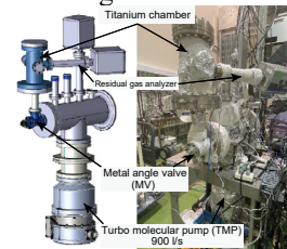
Figure 3: Setup of the build-up test for a titanium vacuum chamber.
