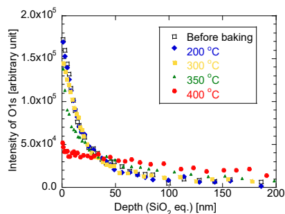
Figure 1: Depth distribution of O1s peak intensity for the samples without baking and baking at each temperature.
