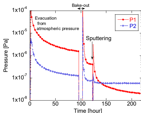
Figure 7: Effect of the surface titanium oxide film removal of the titanium chamber by the sputtering.
