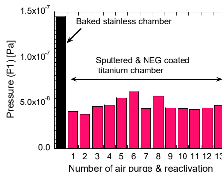
Figure 8: Pressure result after the repeated air purge and reactivation at 200 °C of the titanium chamber whose surface is coated by NEG after surface titanium oxide removal. The pressure of the stainless chamber baked at 200 °C is shown for comparison.
