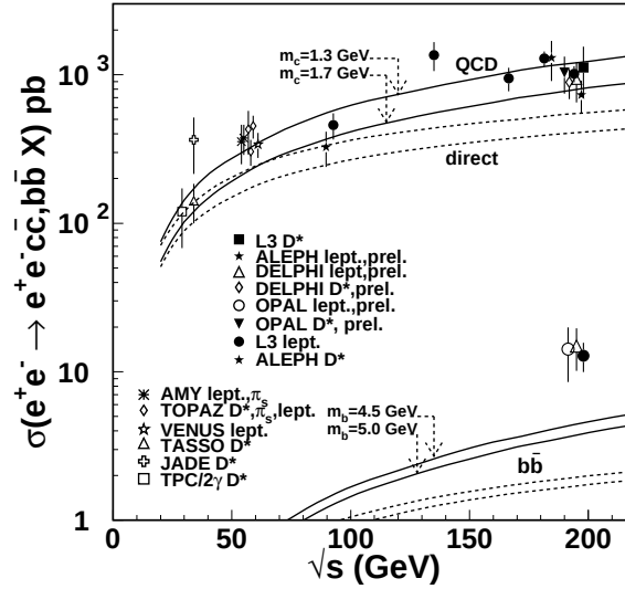
Fig. 1. The open-charm, upper, and open-beauty, lower, production cross sections in photon-photon collisions. The dashed lines correspond to the direct-process contribution only. The effects of a different choice of the values of the quark masses, m_c and m_b , are illustrated.
