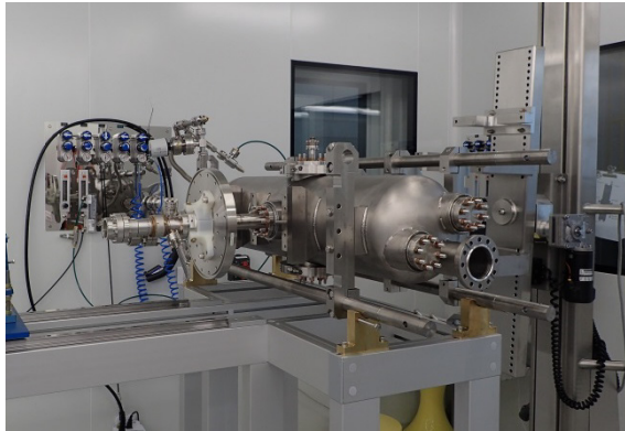
Figure 5: Coupler-cavity assembly.
