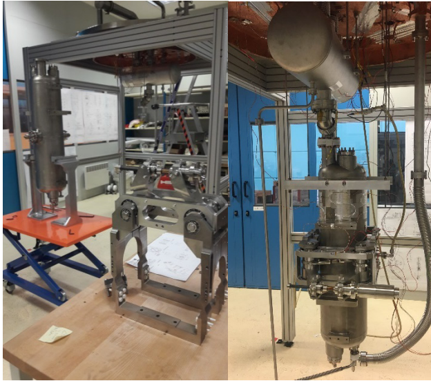
Figure 2: Cavity-tuner assembly.
