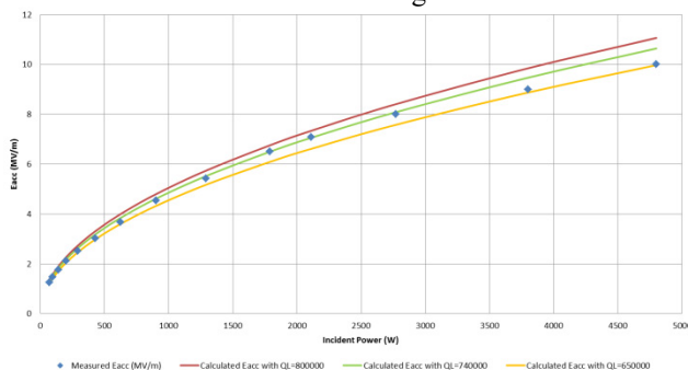
Figure 6: E_{acc} according RF power.
