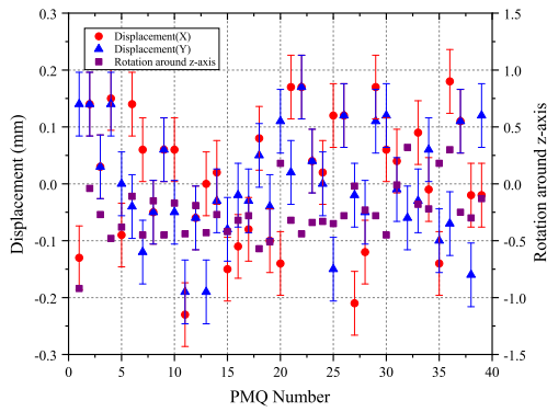
Figure 2: The alignment result of the DTL.
