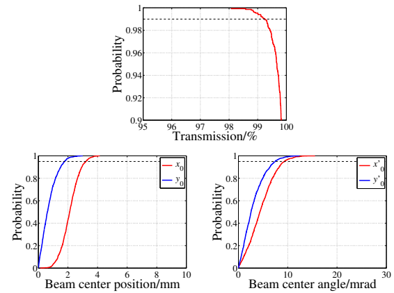
Figure 7: Probability of the transmission rate of the DTL (top), beam center position (bottom-left), beam center angle (bottom-right) at the end of the DTL after changing the input beam.
