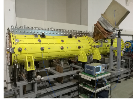
Figure 1: CPHS DTL cavity.
