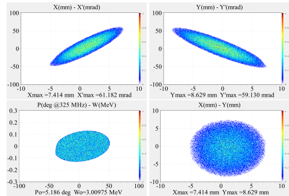
Figure 5: Acceptance of the DTL.
