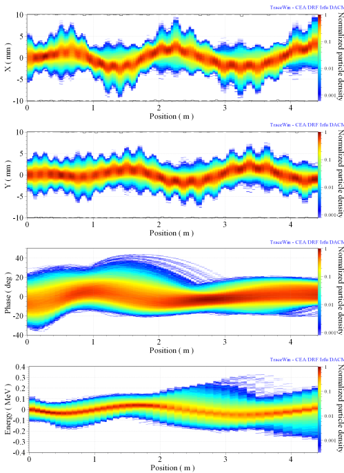
Figure 3: Beam dynamics in the DTL after assembly.
