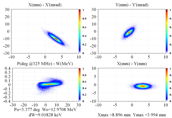
Figure 4: Phase space at the exit of the DTL.
