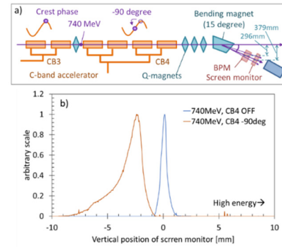
Figure 3: (a) Schematic of the diagnostic system. (b) Typical vertical beam profile, measured at the screen monitor.
