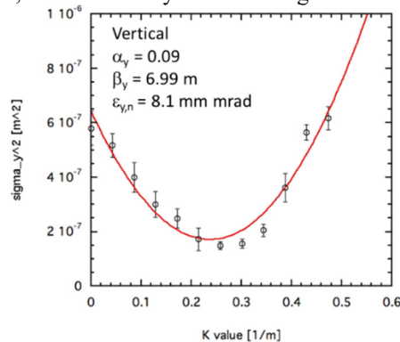
Figure 2: Example of the K-value scan of the quadrupole magnet at the exit of the S-band accelerator. The vertical axis is square of the vertical beam size ( \sigma ) measured at SCM-3 shown in Fig. 1. The error bars mean the statistic error of 10 shots in each data point. The Twiss parameters and the normalized beam emittance are calculated from the quadratic fit (red curve line) of this plot.
