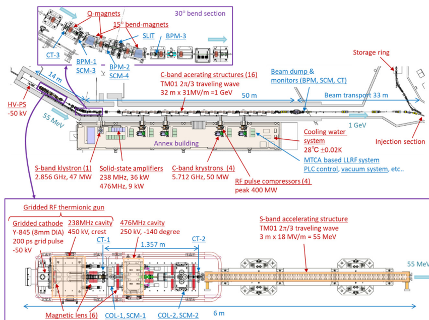
Figure 1: Layout of NewSUBARU injector linac. “COL”, “SCM”, “CT”, “BPM” means a collimator, a screen monitor, a current transformer, and a beam position monitor, respectively.
