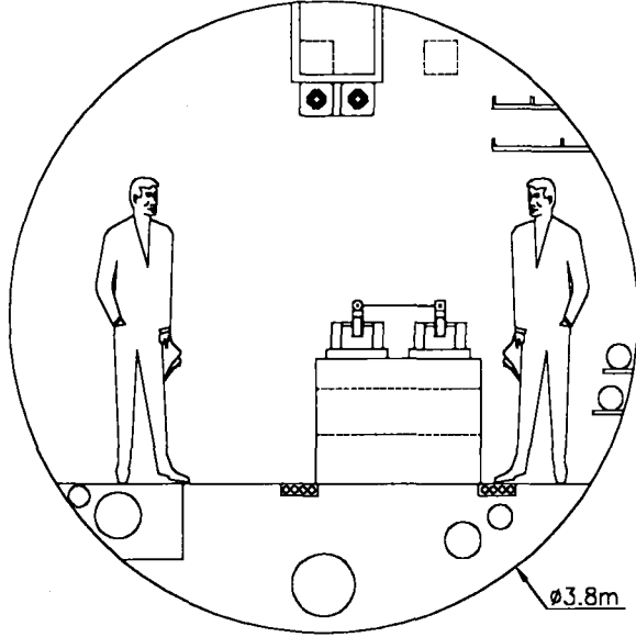
Figure 3: Tunnel cross-section.
