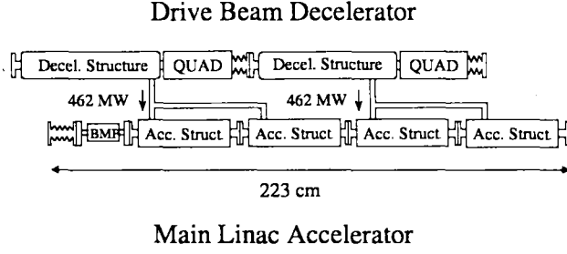
Figure 2: One main beam and drive beam module.
