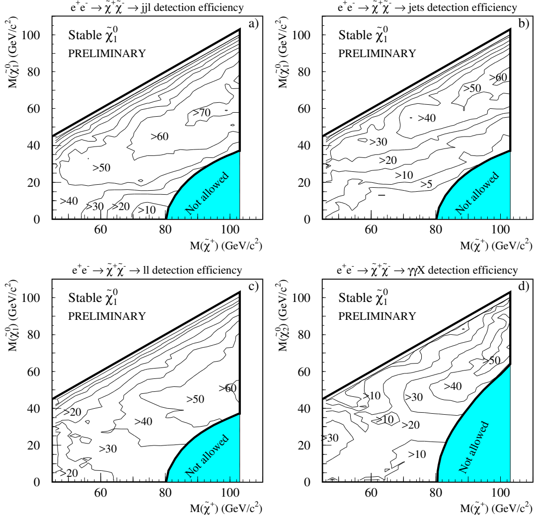
Figure 12: Chargino pair production detection efficiencies (%) for the four decay channels a) jj\ell , b) jets , c) \ell\ell and d) rad , at 206.0 GeV in the (M_{\tilde{\chi}^\pm}, M_{\tilde{\chi}^0}) plane. A stable \tilde{\chi}_1^0 is assumed. The shaded areas are disallowed in the MSSM scheme.
