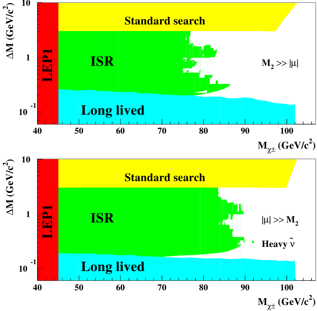
Figure 20: Regions in the plane (M_{\tilde{\chi}_1^\pm}, \Delta M) excluded by DELPHI at the 95% CL using: the standard search for high \Delta M charginos; the search for soft particles accompanied by ISR; and the search for long-lived charginos. The two scenarios are (a) the one in which the lightest chargino is a higgsino and (b) the one in which the lightest chargino is a gaugino. For the second scenario, the limits are valid in the heavy sfermion approximation, while for the higgsino scenario it is sufficient that M_{\tilde{f}} > M_{\tilde{\chi}_1^\pm} .
