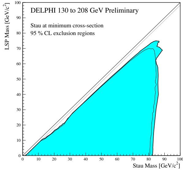
Figure 27: 95% CL exclusion region in the (M_{\tilde{\tau}}, M_{LSP}) plane obtained for the minimal \tilde{\tau}\tilde{\tau}^* pair-production cross-section. The shaded region shows the obtained exclusion limit, and the thin solid line shows the limit expected for no signal events.
