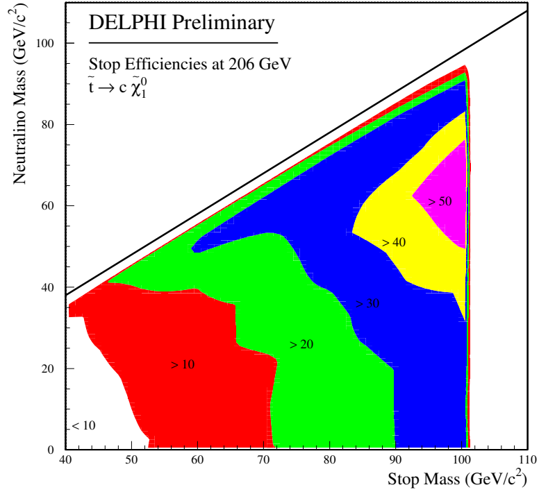
Figure 28: Squark signal detection efficiencies in the plane (M_{q_1}, M_{\tilde{\chi}_1^0}) in the non-degenerate scenario.
