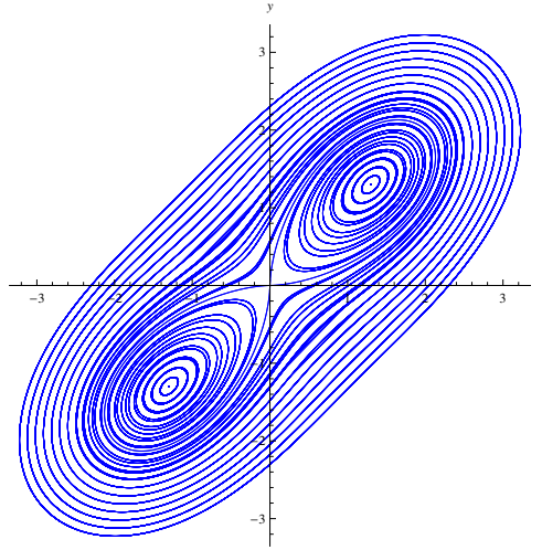
Fig. 1. Duffing-type stable characterization of Gursev instantons for \alpha(AB)^{\frac{1}{3}} = 1 in the phase space; the equilibrium points are \left(-\frac{3\sqrt{3}}{4}, -\frac{3\sqrt{3}}{4}\right) and \left(\frac{3\sqrt{3}}{4}, \frac{3\sqrt{3}}{4}\right) .
