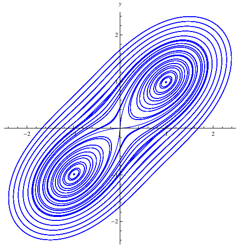
Fig. 2. Duffing-type stable characterization of Gursev instantons for \alpha(AB)^{\frac{1}{3}} = 1.2 in the phase space; the equilibrium points are \left(-\frac{5\sqrt{\frac{5}{2}}}{8}, -\frac{5\sqrt{\frac{5}{2}}}{8}\right) and \left(\frac{5\sqrt{\frac{5}{2}}}{8}, \frac{5\sqrt{\frac{5}{2}}}{8}\right) .
