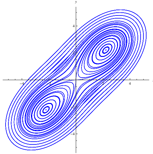
Fig. 3. Duffing-type stable characterization of Gursev instantons for \alpha(AB)^{\frac{1}{3}} = 0.7 in the phase space; the equilibrium points are \left(-\frac{15\sqrt{\frac{15}{14}}}{7}, -\frac{15\sqrt{\frac{15}{14}}}{7}\right) and \left(\frac{15\sqrt{\frac{15}{14}}}{7}, \frac{15\sqrt{\frac{15}{14}}}{7}\right) .
