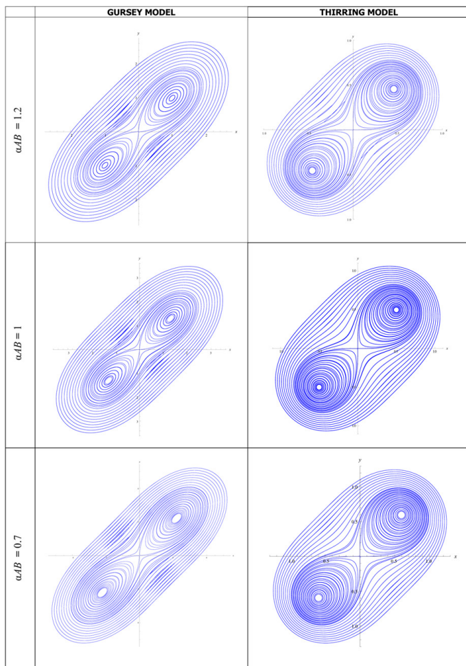
Fig. 4. Dimensionless behaviours of the Gursev and the Thirring instantons in the phase space.
