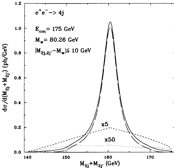
Fig. 5. Distribution of the sum of two invariant masses in the fully hadronic channel at \sqrt{s} = 175 GeV. The chaindot curve corresponds to the two invariant masses from W^{\pm} . The dashed one represents the background (magnified by a factor of 5) from two non-resonant invariant masses in CC11 and MIX43 processes, counted with their multiplicity. The dotted curve corresponds to the NC background (magnified by a factor 50). The solid to signal+total background. For each sum, the two invariant masses lie within 10 GeV from m_W
