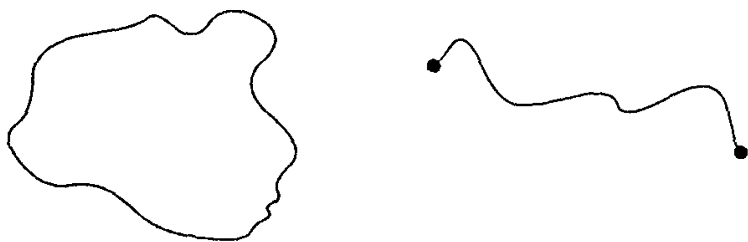
Figure 2. A closed string (left), an open string (right).
