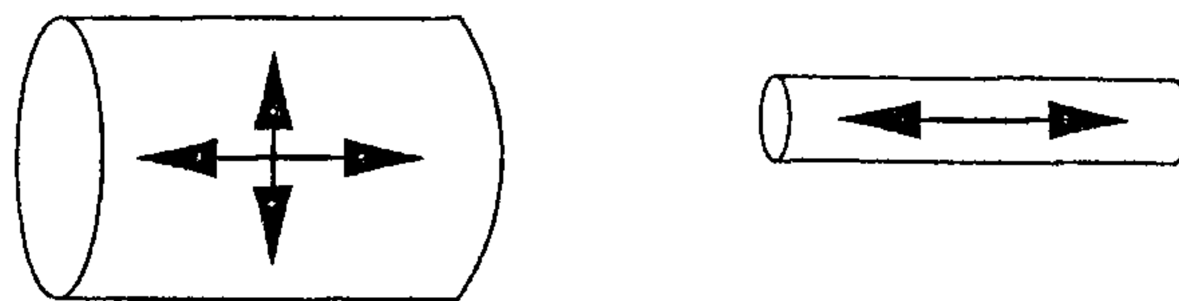
Figure 1. A two-dimensional surface (left) looks one-dimensional when its radius is small (right).
