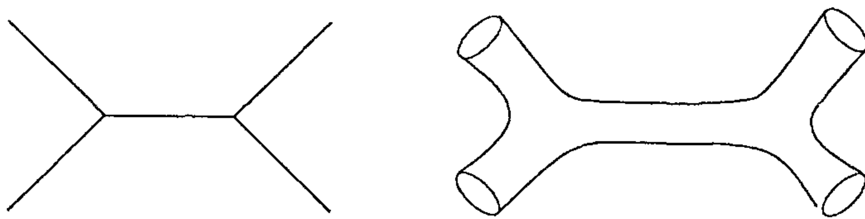
Figure 3. Particle scattering process (left), string scattering process (right).
