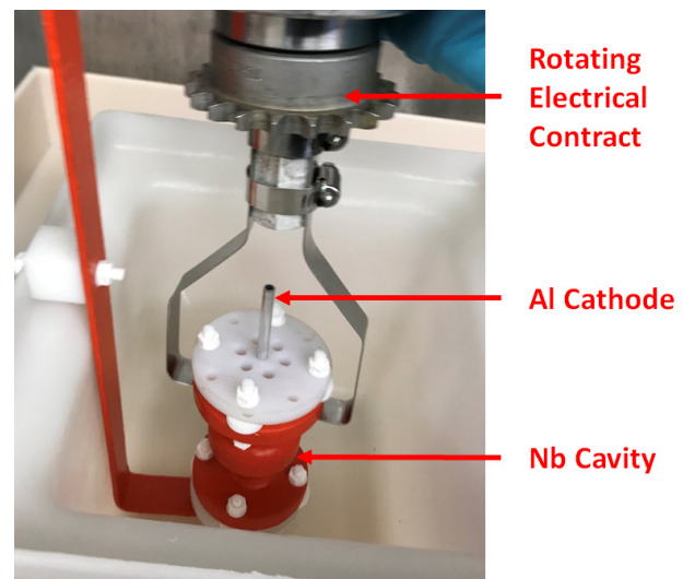
Figure 6: 5 GHz single-cell cavity EP.
