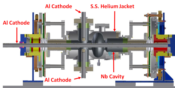
Figure 1: Section view of the EP tool with 1.4 GHz harmonic cavity.
