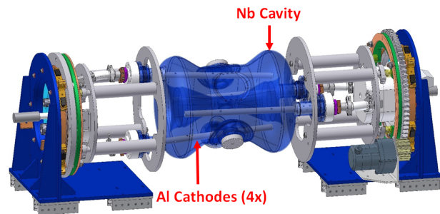
Figure 3: Half-wave cavity in the “low- \beta ” EP tool. Note the stainless steel helium jacket is not shown on the cavity.
