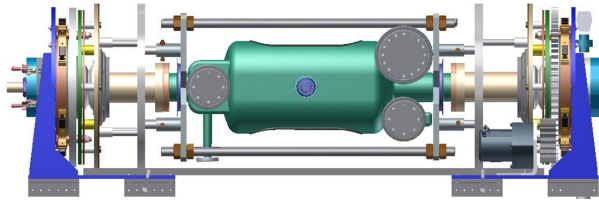
Figure 2: RF-dipole cavity in the “low- \beta ” EP tool.
