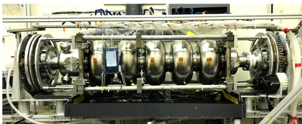
Figure 5: BNL 650 MHz 5-cell cavity in the Argonne “low- \beta ” EP tool.
