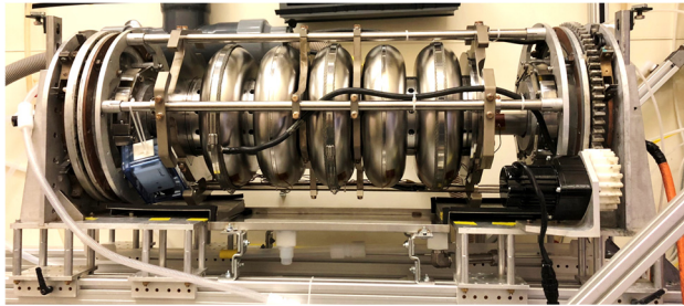
Figure 4: MSU 644 MHz 5-cell cavity in the Argonne “low- \beta ” EP tool. The external water cooling system was installed after this picture was taken.
