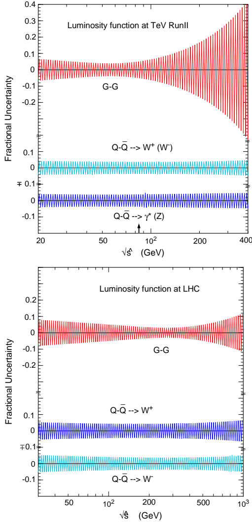
Fig. 2. Uncertainties of the luminosity functions at the Tevatron and at the LHC.
