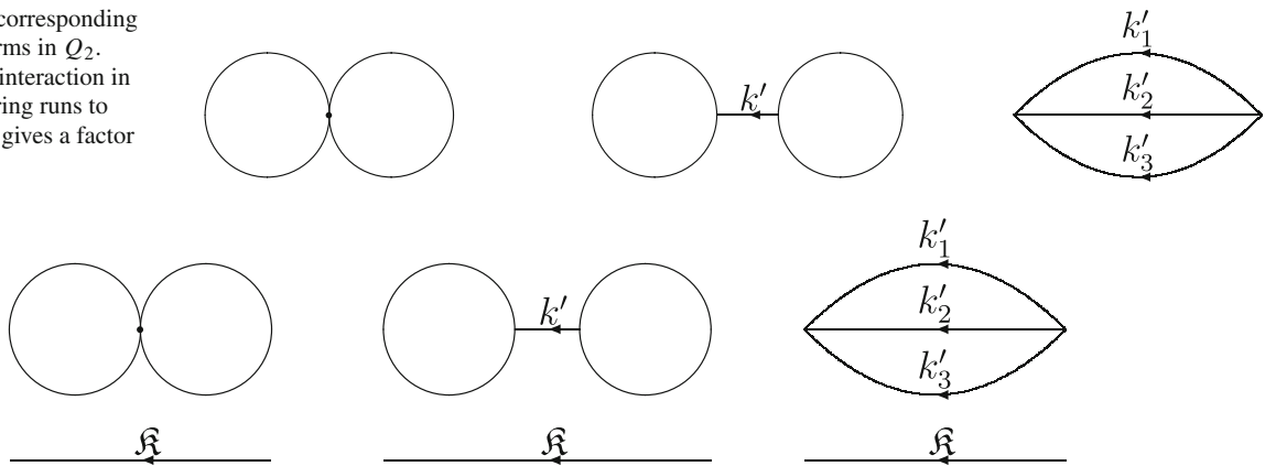
Fig. 2 Diagrams corresponding to the first three terms in the Q_2 2\pi\delta(k_1 - R) contribution to E_2 . The k_1 = R line is disconnected from the diagram. Therefore these are just contributions to the ground
