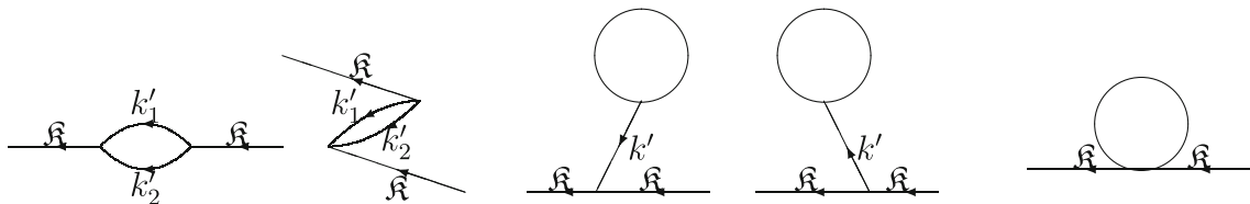
Fig. 3 The first two diagrams give the first term in \mu(R) as written in Eq. (4.12). The next two are equal and yield the second term. The last diagram corresponds to the third term. The other term may be obtained by respectively replacing one k' in the first two diagrams with a zero mode
