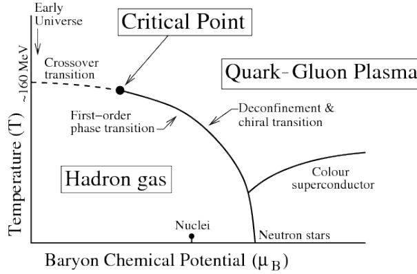
FIGURE II-1: QCD phase diagram [25].
