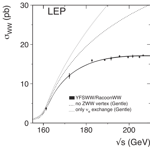
Figure 8.30 Cross section for e^-e^+ \rightarrow W^-W^+ compared with the SM expectation. Also shown is the expectation from t channel \nu_e exchange only, and for the \nu_e and \gamma diagrams only. Reprinted with permission from (Schael et al., 2013).
