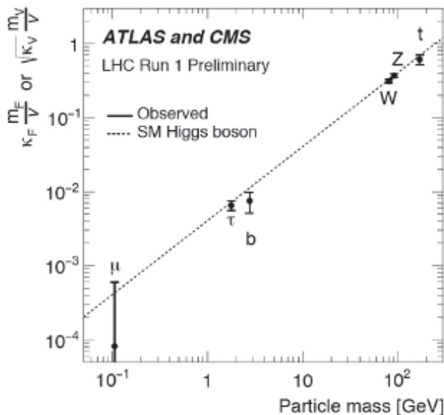
Figure 8.39 Plot of the observed tree-level Higgs couplings to fermions ( \kappa_f m_f/\nu ) and gauge bosons ( \sqrt{\kappa_V} M_V/\nu ) as a function of mass, compared with the SM prediction \kappa_f = \kappa_V = 1 (dashed line). Courtesy of CERN.
