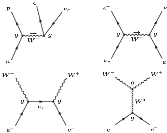
Figure 7.2 Top: intermediate vector bosons mediating \beta decay and \nu_e e^- \rightarrow e^- \nu_e . Bottom left: diagram for e^+ e^- \rightarrow W^+ W^- in the IVB theory. Bottom right: additional diagram in the SU(2) theory.
