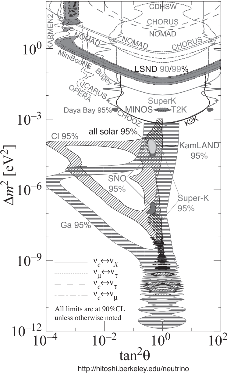
Figure 9.6 Neutrino oscillation results, showing the solar/KamLAND and atmospheric neutrino oscillation regions, the LSND and MiniBooNE regions, and various exclusion regions. Plot courtesy of H. Murayama.
