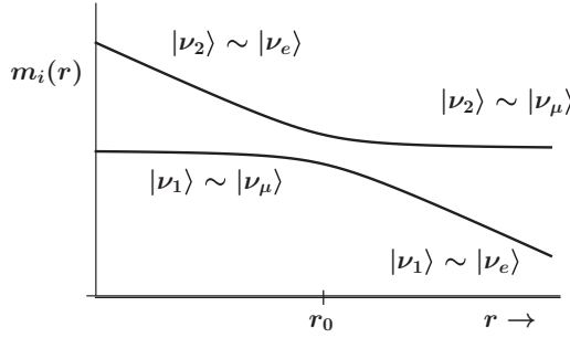
Figure 9.5 A level-crossing (resonance) at r_0 in the presence of matter density that decreases with distance r from the neutrino source. The m_i(r) are the eigenvalues of the matrix in (9.90). (In the full three-neutrino case the state orthogonal to \nu_e is actually a linear combination of \nu_\mu and \nu_\tau .)
