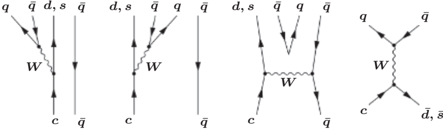
Figure 7.8 Tree-level topological diagrams for D decays, written in terms of an intermediate vector boson W . Gluons may be attached in all possible ways. The first (spectator) diagram represents free quark decay, the second (internal emission) diagram has a reduced color factor (analogous to (5.15)), the third is the exchange diagram, and the last is the annihilation diagram. There are additional one-loop (penguin) diagrams (Section 8.6).
