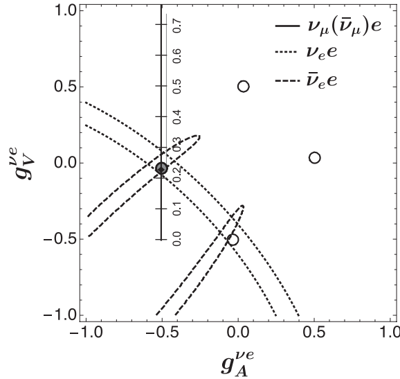
Figure 8.8 Allowed regions in g_V^{\nu e} and g_A^{\nu e} from (\bar{\nu}_\mu^-)e^- , \nu_e e^- , and reactor \bar{\nu}_e e^- elastic scattering, compared to the predictions of the SM as a function of \sin^2 \theta_W in the \overline{MS} scheme. The SM best fit (shaded area) is almost identical to the experimental region. The \nu_\mu e regions are at 90% c.l., and the bands are at 1\sigma . Plot courtesy of the Particle Data Group (Patrignani, 2016).
