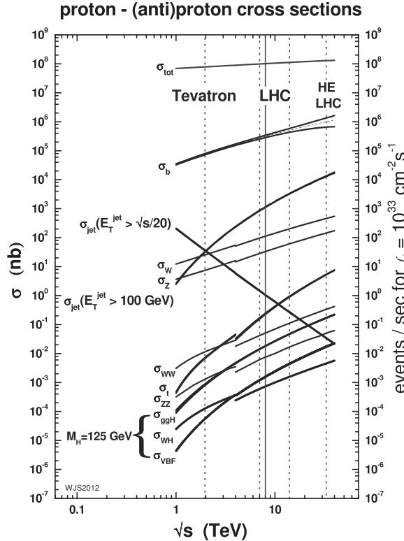
Figure 6.2 pp and p\bar{p} cross sections for SM processes as a function of energy, with LHC energies of 7, 8, and 14 TeV indicated. HE LHC refers to a possible 33 TeV high-energy upgrade. The discontinuities are due to the use of p\bar{p} ( pp ) at lower (higher) energies. Plot courtesy of W.J. Stirling, private communication.
