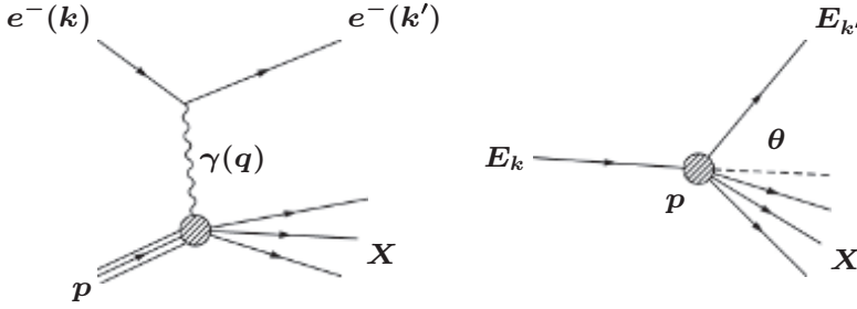
Figure 5.11 Left: deep inelastic scattering e^-p \rightarrow e^-X , where X represents unobserved hadrons. q = k - k' is the four-momentum of the virtual photon. Right: kinematics in the proton rest frame. E_k and E_{k'} are the energies of the initial and final electrons, and \theta is the laboratory scattering angle.
