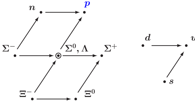
Figure 7.4 Weight diagrams for the baryon octet and for the quarks. The hadronic charge raising current J^{h\dagger} mediates transitions to the right ( \Delta S = 0 ) or diagonally up and to the right ( \Delta S = \Delta Q ), but not diagonally up and left (FCNC) or to non-adjacent states ( \Delta S = -\Delta Q ).
