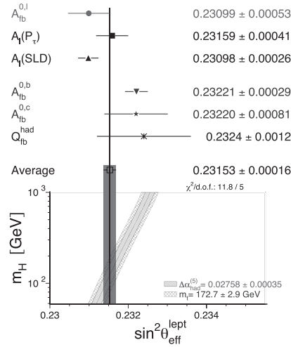
Figure 8.25 \bar{s}_\ell^2 from various leptonic and hadronic asymmetries, compared with the SM predictions as a function of M_H using the observed M_Z . Reprinted with permission from (Schael et al., 2006a).
