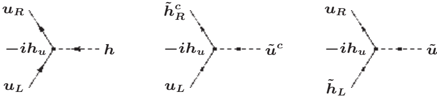
Figure 10.5 Yukawa vertices from (10.107). There are three more diagrams in which the incoming and outgoing particles are reversed.
