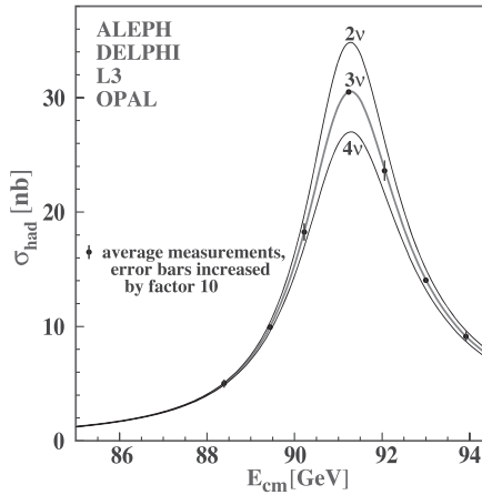
Figure 8.23 Lineshape for Z \rightarrow \text{hadrons} , compared with the expectation for 2, 3, and 4 ordinary neutrinos lighter than \sim M_Z/2 . The asymmetry is due to the explicit factor of s in the numerator of the Breit-Wigner formula (cf. Equation F.7) and to radiative corrections. Reprinted with permission from (Schael et al., 2006a).
