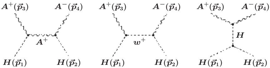
Figure 4.3 Tree-level diagrams for HH \rightarrow A^+A^- in an R_\xi gauge. There are two additional u -channel diagrams obtained from the first two by p_1 \leftrightarrow p_2 ,
