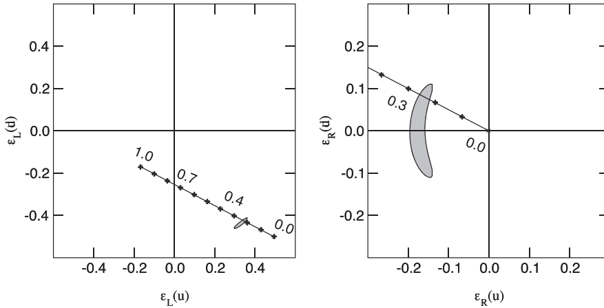
Figure 8.11 90% c.l. allowed regions in \epsilon_{L,R}^{\nu h}(u) vs \epsilon_{L,R}^{\nu h}(d) from (\bar{\nu}_\mu^-)N elastic, exclusive inelastic, and deep inelastic scattering, compared to the predictions of the SM as a function of \sin^2 \theta_W , updated from (Amaldi et al., 1987).
