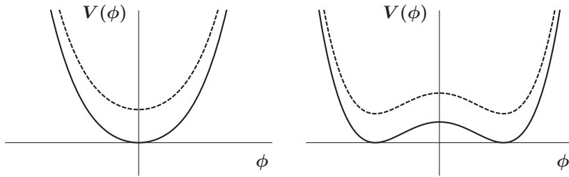
Figure 10.4 Left: potentials which preserve internal symmetries. Right: potentials which break internal symmetries. In both cases, supersymmetry is preserved for V|_{\min} = 0 (solid) and spontaneously broken for V|_{\min} > 0 (dashed).
