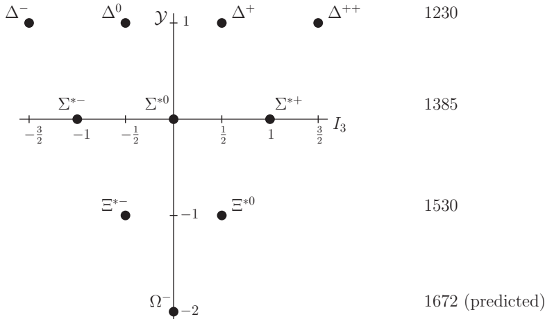
Figure 3.2 Weight diagram for the J^P = \frac{3}{2}^+ decuplet.
