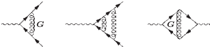
Figure 8.20 QCD corrections to the Wq\bar{q} or Zq\bar{q} vertices and mixed corrections to an electroweak self-energy diagram.
