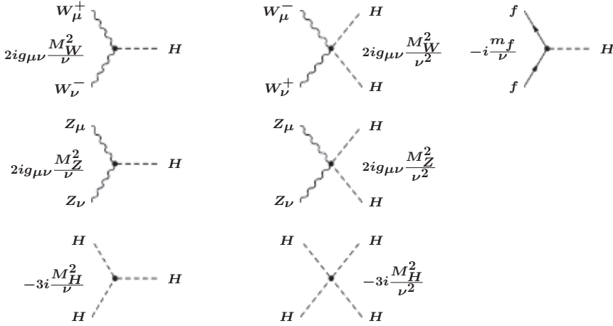
Figure 8.3 Higgs interaction vertices in the standard model.
