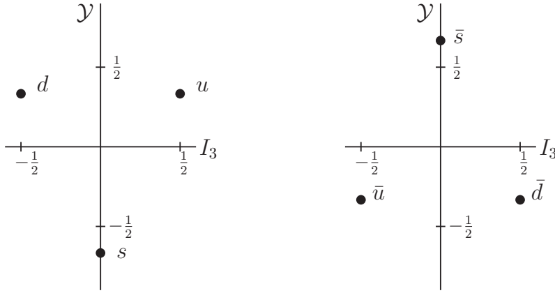
Figure 3.3 Weight diagrams for the 3 and 3^* of SU(3) .
