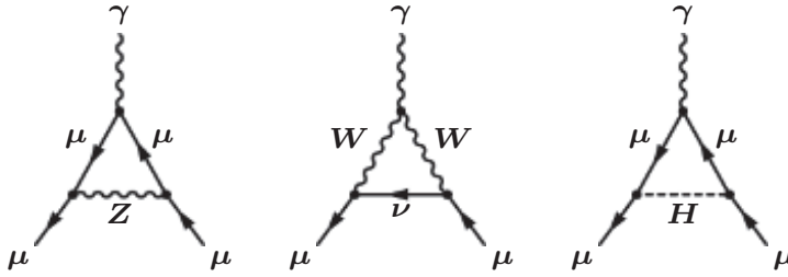
Figure 2.20 One-loop electroweak contributions to a_\mu = (g_\mu - 2)/2 .
