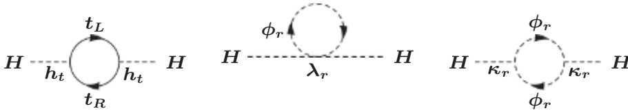
Figure 10.3 t quark and \phi_r contributions to M_H^2 .
