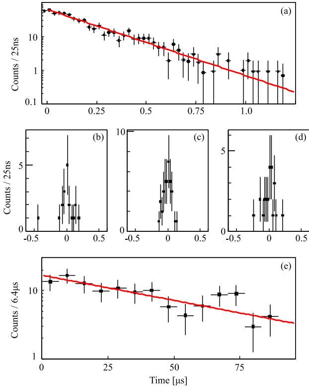
Fig. 2. (a): Time spectrum ( t_\gamma ) of the 757-keV \gamma ray in ^{125}\text{Pd} . (b): Time difference spectrum ( \Delta t_{\gamma\gamma} ) of the 115-keV \gamma ray relative to the 108-keV transition in ^{125}\text{Pd} . (c) and (d): Sum of \Delta t_{\gamma\gamma} of the 757- and 825-keV \gamma rays relative to the 115- and 108-keV transitions in ^{125}\text{Pd} , respectively. (e): t_\gamma of the 422-keV \gamma ray in ^{127}\text{Pd} . In the panels (a) and (e), the red solid lines represent the results of a log-likelihood fit.
