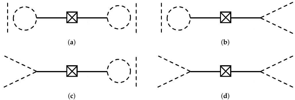
Figure 2. Diagrammatic representations of the terms contributing to \rho_{0,2;0,2}(t) , as given in Equation (59); the crossed box depicts the insertion of the initial density matrix element and solid/dashed lines represent \phi/\varphi -propagators. (a) shows two \phi -propagators ending in \varphi -tadpoles, while two propagators at equal time but different positions appear. (b,c) each depict one \phi -propagator ending in a \varphi -tadpole and one propagator at equal time but different positions appearing, and, in addition, another \phi -propagator decaying into two \varphi -particles. (d) shows two \phi -propagators each decaying into two \varphi -particles.
