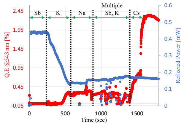
Figure 1: QE (red) and reflected power (blue) during deposition of cathode NaKSb(Cs)-2. The incident power @ 543 nm during photocathode growth was 1.9 mW.
