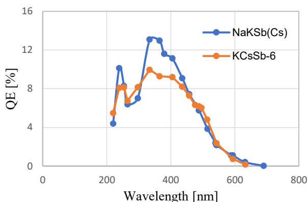
Figure 2: NaKSb(Cs)-2 photocathode spectral response.
