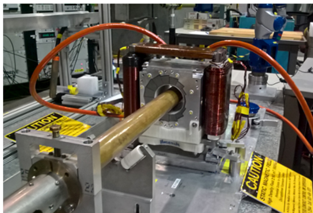
Figure 2: Magnet measurements of the 'CBETA' magnets.
