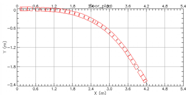
Figure 6: Layout of the first achromatic permanent magnet proton gantry module.
