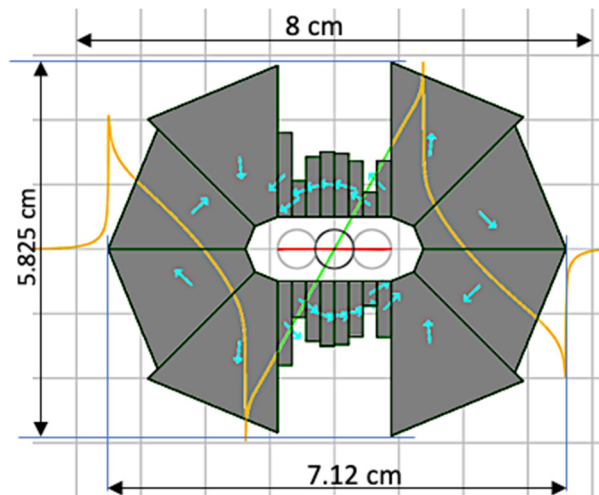
Figure 3: Initial permanent magnet gantry design with quadrupole gradient of 150 T/m.
