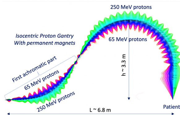
Figure 7: Orbits throughout the whole proton gantry up to the patient.
