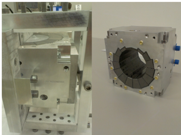
Figure 1: Assembly tools (left) built by 'KYMA' and the assembled combined function permanent magnet (right).
