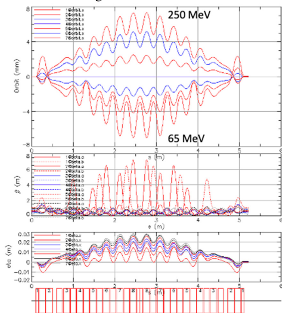
Figure 5: Lattice functions in the first achromatic gantry module with proton orbits between 65-250 MeV.
