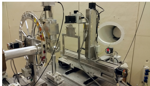
Figure 5: Photograph of the setup for heavy ion irradiations.
