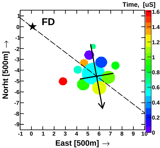
Fig. 3: Footprint of a Monte-Carlo event. Each circle represents an infill array counter. Circle area is proportional to the logarithm of the counter pulse height in VEM, circle color represents the counter time in \mu\text{S} , black arrow shows the reconstructed event direction, and the dashed line is the intersection of the reconstructed shower-detector (MD/TALE FD) plane and ground. Star represents the location of the MD/TALE FD.
